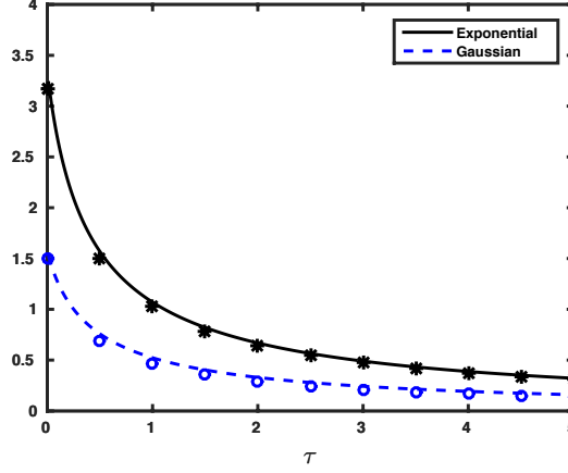
Figure 1: Comparison of the exact formula for the minimal wave speed as given in (3.3) with direct numerical simulations for the nonlinearity S in (3.5) and two different exponentially bounded kernels. The black line corresponds to the theoretical wave speed prediction in the case of \mathcal{K}(x) = e^{-|x|}/2 and the stars are direct numerical simulations. The blue dashed line corresponds to the theoretical wave speed prediction in the case of \mathcal{K}(x) = e^{-x^2}/\sqrt{\pi} and the circles are direct numerical simulations.
