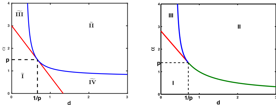
FIG. 2.2. Differences between the speeds s_{\text{lin}}(p) (left) and s_{\text{sel}}^{\text{KPP}}(p) (right) with p=1.5 . On the domains I and \tilde{I} both speeds are equal to 2. On the domains II and \tilde{II} both speeds are equal to 2\sqrt{d\alpha} . On domains \tilde{III} , \tilde{IV} and III both speeds are equal to s_{\text{anom}} > \max(2, 2\sqrt{d\alpha}) . Notice that when considering the selected speed s_{\text{sel}}^{\text{KPP}}(p) for the full system (1.1), the domain \tilde{IV} disappears, and in that region of parameters the selected speed is simply equal to \max(2, 2\sqrt{d\alpha}) .
