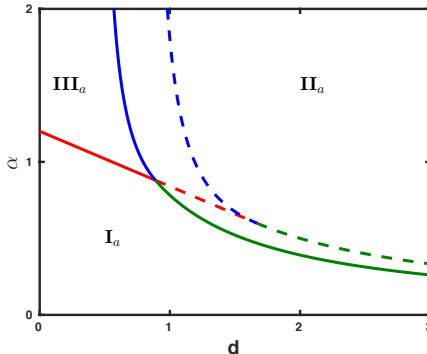
FIG. 4.1. Selected speed of (1.1) with f(u) = \alpha u(1-u)(1+au) , p=0.6 , a=5.5 as stated in Conjecture 2. The domain \widetilde{\text{I}}_a corresponds to s_{\text{sel}}^m(p) = 2 , the domain \widetilde{\text{II}}_a corresponds to s_{\text{sel}}^m(p) = s_0 , and the domain \widetilde{\text{III}}_a corresponds to the anomalous speed s_{\text{sel}}^m(p) = s_{\text{anom}} > \max(2, c_0) . The dotted lines represent the shifted boundaries of the domains when a \leq 2 , that is when s_{\text{sel}}^m(p) is linearly determined (see Conjecture 1). In that case, the respective domains do not depend on a \in (0, 2] .
