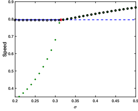
Figure 2: Numerically computed wave speeds of the u -component, black circles, and of the v -component, green plus sign for \epsilon = 1 in (2.5). The horizontal blue line s = s^* = \sqrt{2}(a + 1/2) represents the sign of the associated principal eigenvalue of the operator H_\sigma and the red diamond indicates the critical value \sigma^* at which this principal eigenvalue vanishes. The solid part of the line indicates a negative principal eigenvalue while the dashed part indicates a positive one. Here, \sigma^* \simeq 0.314 . For all numerical simulations we have set a = 1/16 .
