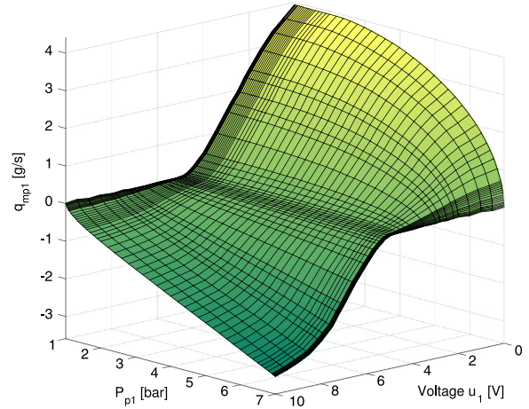
Fig. 5. Characterization map of a Festo MYPE5 servovalve.
