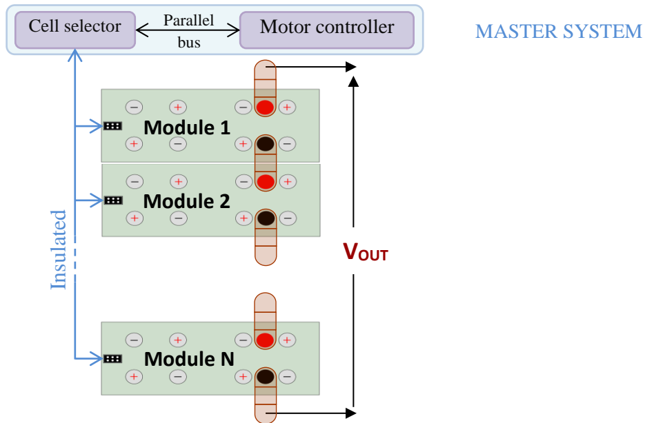
Figure 9 : Serial arrangement of modules of prototype 2
