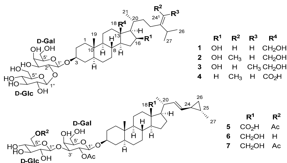
Figure 1. Structure of poecillastrosides A–G (1–7).
