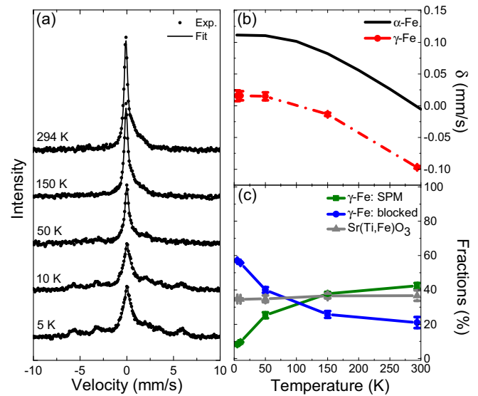
FIG. 7. (a) Conversion electron Mössbauer spectroscopy (CEMS) data and fit measured at different temperatures (5–294 K). (b) The measured isomer shift corresponding to \gamma -Fe, compared to that of \alpha -Fe, measured in the same setup on a 20-nm \alpha -Fe film deposited on Si. (c) The fractions of the different components: \gamma -Fe in the blocked regime, \gamma -Fe in the superparamagnetic (SPM) regime, nonprecipitated Fe in \text{Sr}(\text{Ti},\text{Fe})\text{O}_3 (the fit model is described in Supplemental Material [42]).
