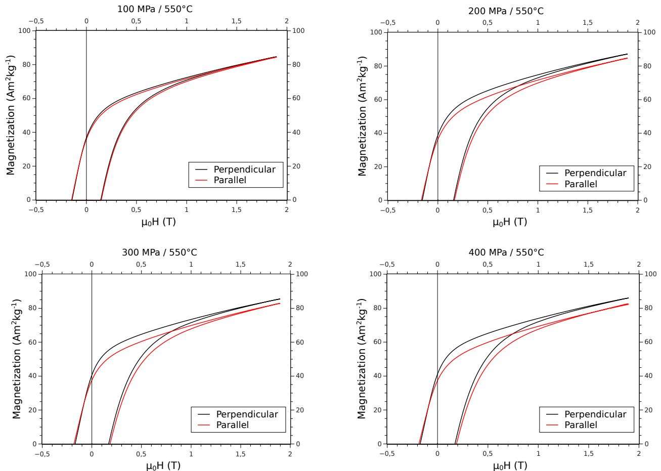
FIG. 2. Magnetization ( \text{A m}^2 \text{kg}^{-1} ) versus \mu_0 H_c (T) of the samples sintered at 550^\circ \text{C} and 100, 200, 300 and 400 MPa, measured parallel and perpendicular to the sintering pressure direction.
