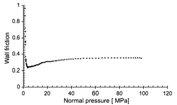
Fig. 5. Wall friction coefficient versus normal pressure (from die compaction experiments).
