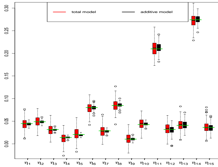
Figure 1: Boxplot of 1000 estimates of the 15 Shapley effects using the two methods suggested: with a total model in red and with an additive model in black. We also represent the true values of the Shapley effects with green horizontal segments.
