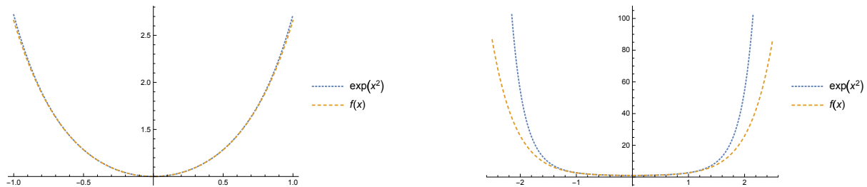
Figure 1: Superimposed curves of \exp(x^2) and f(x) for x \in [-1, 1] in the first graphic, and for x \in [-2.5, 2.5] in the second graphic.
