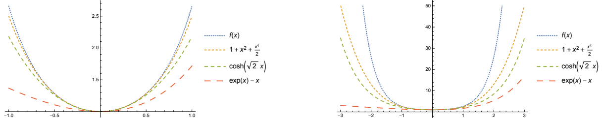
Figure 2: Superimposed curves of f(x) , 1 + x^2 + x^4/2 , \cosh(\sqrt{2}x) and \exp(x) - x for x \in [-1, 1] in the first graphic, and for x \in [-3, 3] in the second graphic.
