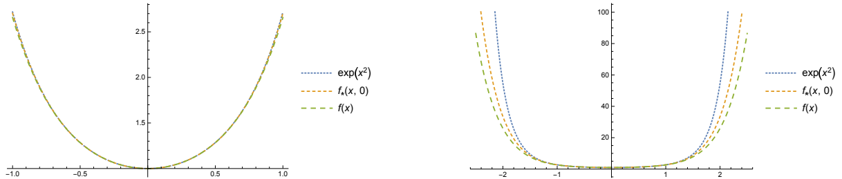
Figure 3: Superimposed curves of \exp(x^2) , f_*(x; n) for n = 0 and f(x) for x \in [-1, 1] in the first graphic, and for x \in [-2.5, 2.5] in the second graphic.
