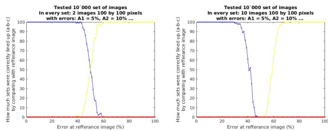
Fig. 1. Influence of reference classifier quality on classifier comparison
