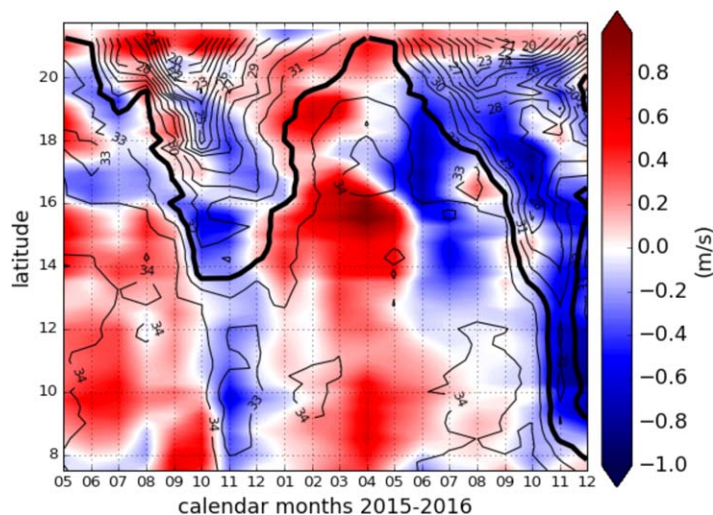
Figure 6. May 2015 to December 2016 latitude-time sections of average monthly alongshore currents within 200 km of the East Indian coast (region delimited by a magenta contour on Figure 5a). The average SSS are represented as contours (contour interval: 1 pss; bold 32 pss contour). Currents are shown as positive when they flow toward the North of the bay.
