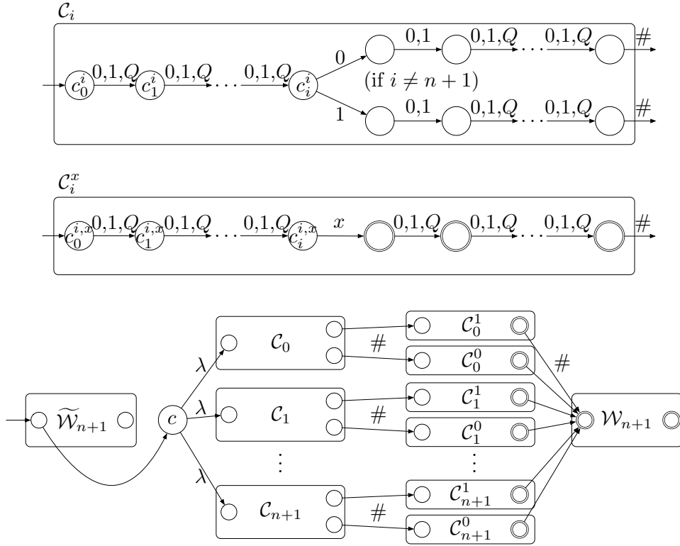
Figure 10: \mathcal{E}_{local} accepts words that include two consecutive configurations where the tape changes in a position that did not have the head of M over it. \tilde{W}_{n+1} is like W_{n+1} , but with an empty set of final states. C_i and C_i^x have lengths of n+2 , reading configurations of n+1 characters.
