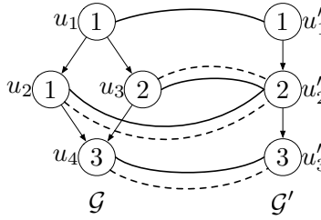
Figure 4: Two data graphs with same label in all edges (not shown). The dotted lines represent the maximal bisimulation for \text{XPath}_= . The solid lines represent an ML-bisimulation when data is absent.
