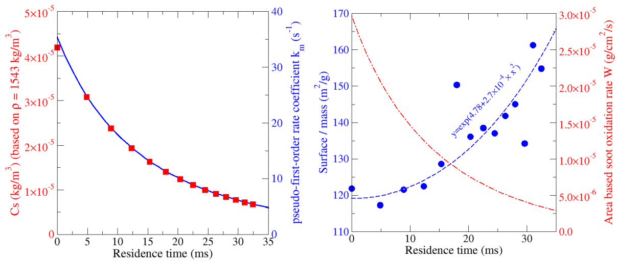
A: Mass concentration deduced from LII measurement (red plain boxes) and determined pseudo-first-order rate of the oxidation process based on mass (blue plain curve).
