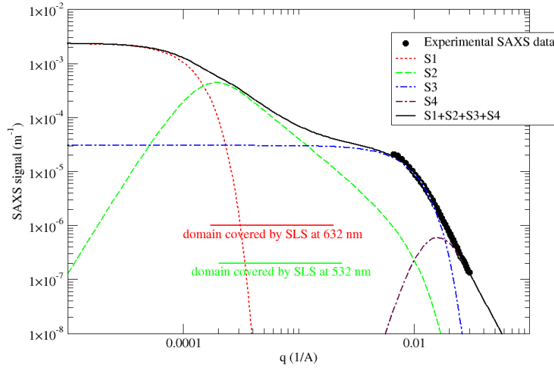
FIG. 5 Example of SAXS theoretical modeling corresponding to the experimental measurement at HAB = 2 \text{ mm} , \bar{N}_p = 75 , D_{p,geo} = 26.4 \text{ nm} , \sigma_{p,geo} = 1.34 , f_v = 20.0 \text{ ppb} , \rho_e = 3.59 \times 10^{27} \text{ m}^{-3} , I_e = 7.94 \times 10^{-30} \text{ m}^2 , PDI_a = 2 , D_f = 1.73 , p = 4 ).
