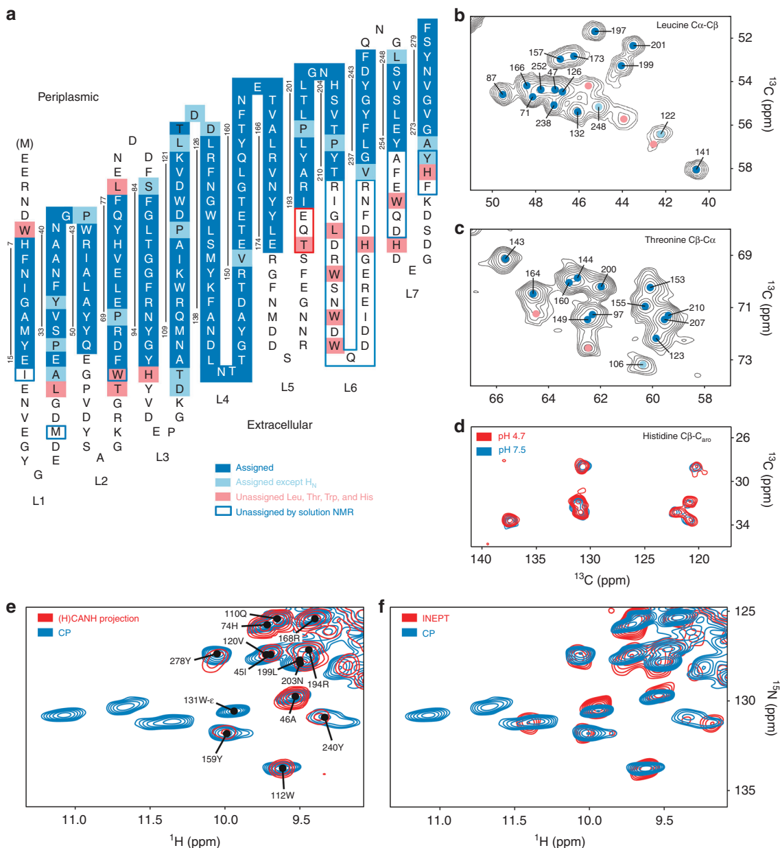
Fig. 1 Resonance assignment and OmpG topology. Assigned residues are indicated in blue. a For residues in light blue, the ^1H_N shift is unknown but partial carbon assignment was obtained. Pink indicates unassigned residues as discussed in the text. Residues in blue frames do not show signals in solution NMR spectra and residues in the red frame were assigned by solution NMR but not solid-state NMR, see text. Vertical lines indicate the \beta -strands with residue numbers. b-d Spectral regions of ^{13}C - ^{13}C correlation spectra comprising C\alpha - C\beta peaks of b leucine in the GAVLS(W) sample (20 ms DARR), c threonine in a DARR spectrum of the 1,3-TEMPQANDSG sample (50 ms mixing), and d histidine in a 50 ms DARR spectrum of the GANDSH(LV) sample. For the peaks indicated by pink dots in these ^{13}C - ^{13}C spectra, no strip could be found in the ^1H -detected 3D spectra. e, f Overlays of a CP-based ^1H - ^{15}N -correlation (blue) comprising the region of Trp side chain cross peaks with the projection of the CANH spectrum ( e ) and an INEPT-based HSQC ( f )
