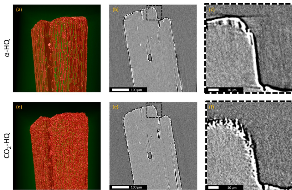
Figure 5. X ray tomography images of a single \alpha HQ crystal (top) and of the same crystal after enclathration with \text{CO}_2 (bottom): (a, d) 3D view in false color of the top of the crystal, (b, e) longitudinal cross section, and (c, f) zoom on a region of interest of b and e.
