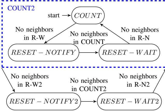
Fig. 5: Finite State Machine Component for EBET ( k = 2 )
