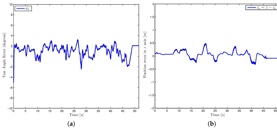
Figure 11. Quad-rotor’s yaw and z axis error stabilization. (a) Quad-rotor’s yaw error stabilization; (b) Position error in the z axis.
