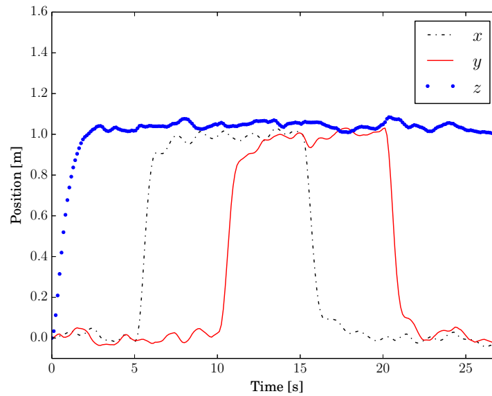
Figure 6. Quad-rotor’s translation responses.
