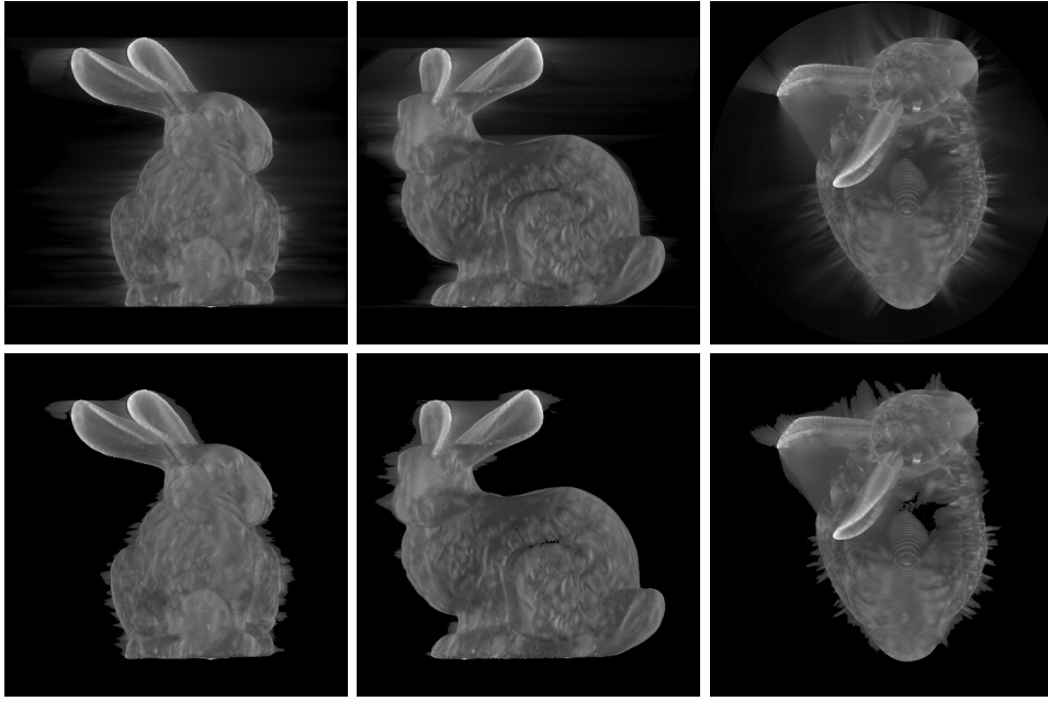
FIGURE 13. Reference reconstruction: full volume of size 512^3 (top), and extraction of 0.05 \cdot 512^3 voxels (bottom).
