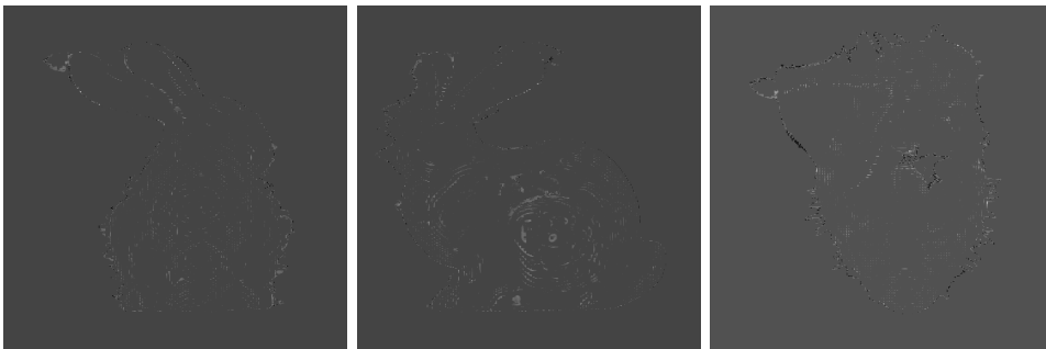
FIGURE 12. Greedy MIP subtracted from the reference MIP, for \alpha = 5\% .
