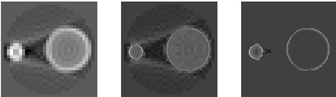
FIGURE 5. Multiresolution reconstruction for Figure 3: initialization of size 32^2 (left), multiresolution image (middle), and the 0.05 \times 256^2 thinnest pixels (right).
