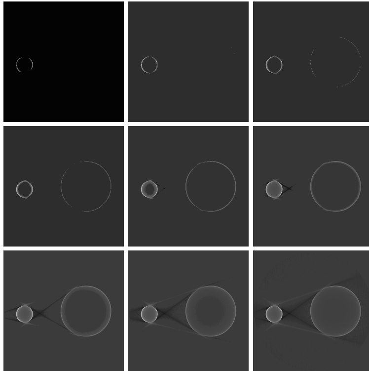
FIGURE 8. Reconstructions of \alpha 512^2 pixels for the scene of Figure 6, with initialization of size 128^2 and \alpha = 0.32 \cdot 2^\beta ; -8 \leq \beta \leq 0 increases in the usual reading order.
