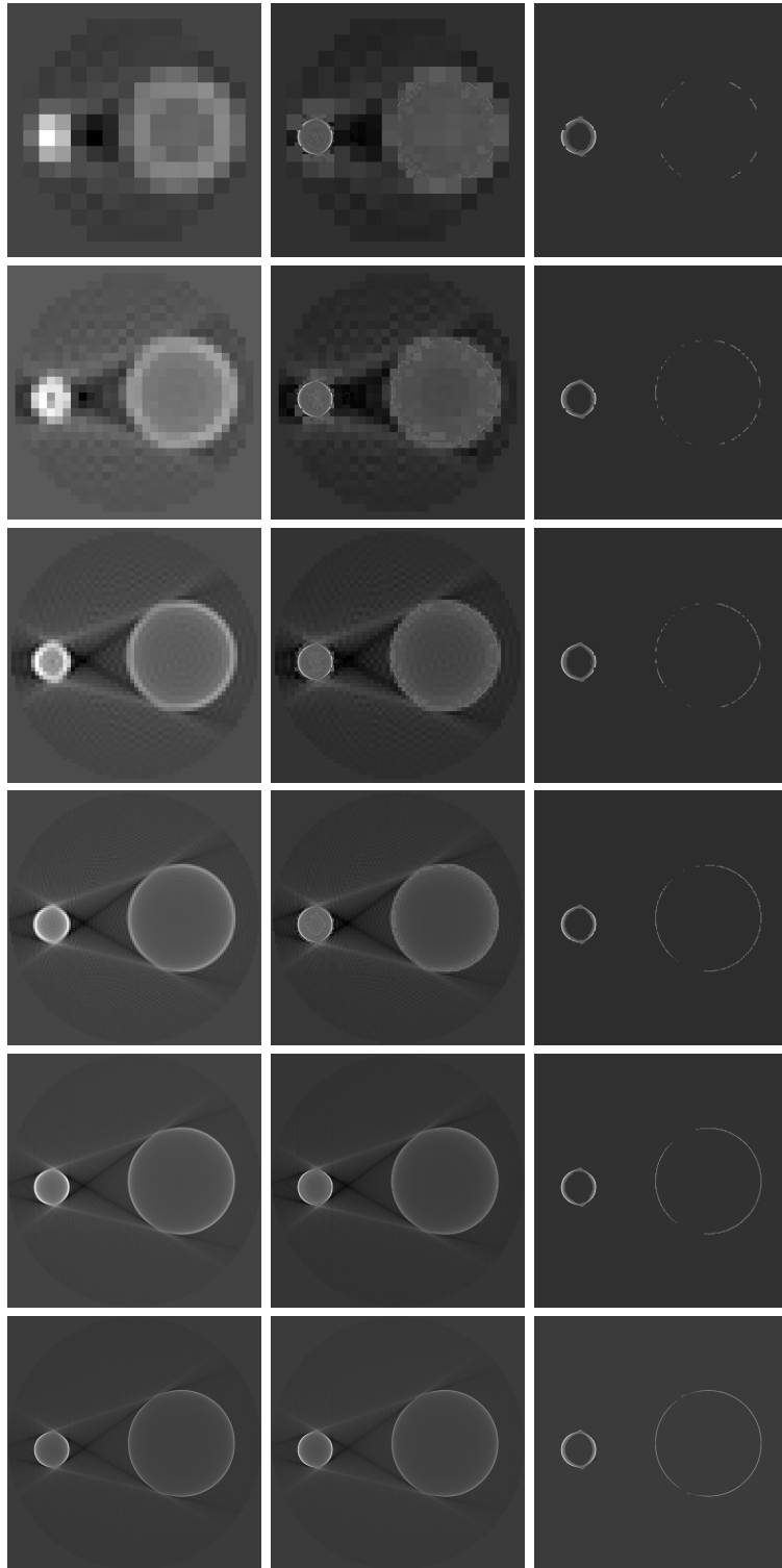
FIGURE 7. Reconstructions for the Figure 6: coarse initialization of size (2^{k_0})^2 (left), multiresolution reconstruction (middle), and the thinnest pixels (right). From top to bottom: k_0 = 4, 5, 6, 7, 8 ; on the last line: reference reconstruction.
