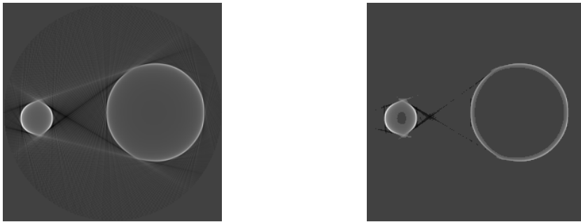
FIGURE 4. Reference for the reflectogram of Figure 3: full reconstruction of size 256^2 (left), and after extraction of 5% of the pixels (right).
