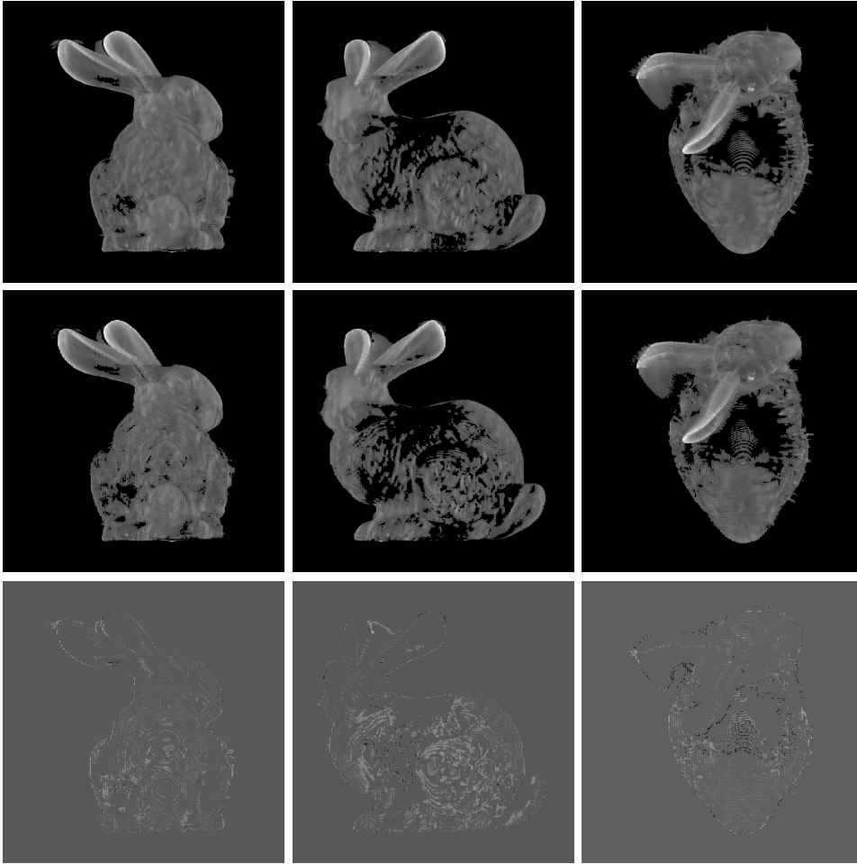
FIGURE 15. Reference reconstruction, greedy reconstruction (initialization 128^2 \cdot 512 ), and difference between the two; \alpha = 1\% .
