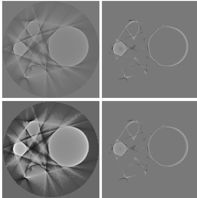
FIGURE 10. Reconstructions for the Figure 9: top, reference before and after extraction; bottom, initialization and final reconstruction by the multiresolution method.
