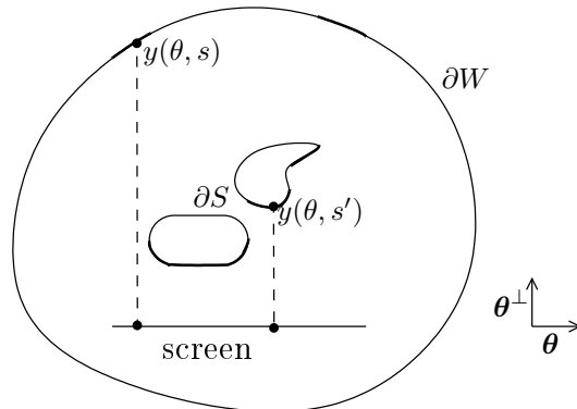
FIGURE 1. Reflective projection for an angle \theta \in \Theta : the wall \partial W and the scene \partial S are projected in the direction -\theta^\perp on a screen, along the rays x \cdot \theta = s, s \in [-R, R] . The set of the projected visible points, y(\theta, s), s \in [-R, R] , is represented in bold. The dashed lines represent two rays of projection, from the visible points y(\theta, s) and y(\theta, s') , to the screen.
