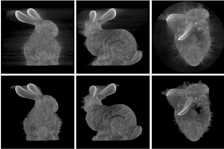
FIGURE 14. Greedy reconstruction: initialization of size 128^2 \cdot 512 , and reconstruction at 5%.
