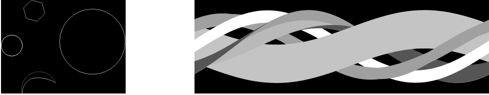
FIGURE 9. Scene (left) and its reflectogram 3217 \times 1024 (right).
