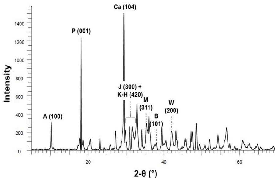
FIGURE 3 | XRPD pattern of hydrothermally oxidized steel slag (300°C–190 bar, APW-300C ), the most intense peak of every identified crystalline phases is labeled (see Table 2 ) as follows: hydroxylapatite (A), portlandite (P), calcite (Ca), jaffeite (J), katoite-hibschite series (K-H), magnetite (M), brucite (B), and wüstite (W).
