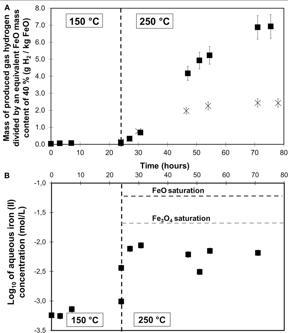
FIGURE 7 | Time-resolved monitoring of (A) the H 2 gas production (squares) and (B) the ferrous concentration of the hydrothermal oxidation of decalcified steel slag from 150 to 250°C at 180 bar in presence of 1 M acetic acid (APAc-1M-250C). H 2 gas production was monitored in a previous run performed under the same working conditions but without steel slag sample (crosses). Hydrogen production data were normalized to an equivalent FeO content of 40%, i.e., in accordance with \mu XRF analysis on calcium depleted sample. Fe 2+ concentration at saturation were calculated using Phreeqc with Ilnl.dat database under the conditions of the experiment. At 150°C, Log 10 (Fe 2+ aq , mol/L) at saturation were found to be equal to -0.4 for FeO and -0.6 for Fe 3 O 4 and are not shown.
