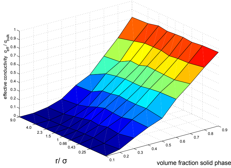
Fig. 17 Parameter study of the effective conductivity of the model described in Section 4.2.
