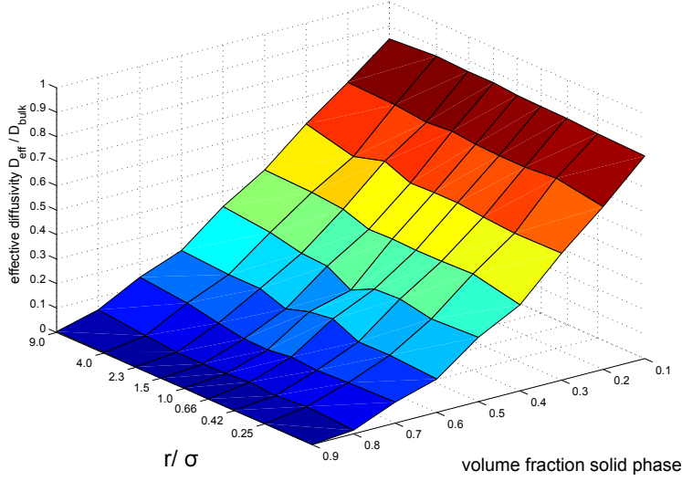
Fig. 18 Parameter study of the effective diffusivity of the model described in Section 4.2.
