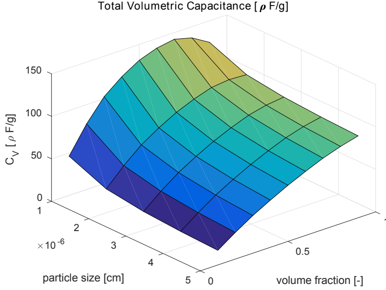
Fig. 20 Parameter study of the total capacity of a structure of the model described in Sect. 4.2, with spheres of radius d , the volumetric and areal capacities from Eq. 32 and \frac{r}{\sigma} = 1.5 .
