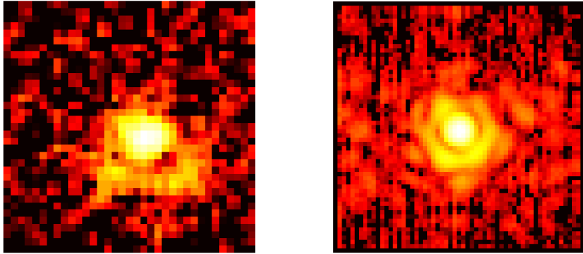
Figure 1. Left: An image acquired by the DTTS imager on SPHERE during a night with a strong low wind effect, shown in log-scale (courtesy of J.F. Sauvage). The asymmetric ‘ear’ like features on the PSF shown here are an example of the PSF contamination experienced throughout the course of the entire night, and restrict the use of the instrument. Right: A K-band, short exposure Keck/NIRC2 image (also shown in log-scale) displaying typical features of ‘low order residuals’, which are persistent throughout the duration of the closed AO loop (courtesy of S. Ragland).
