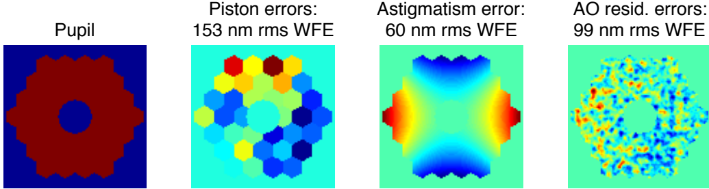
Figure 7. From left to right: Keck pupil, simulated piston phasing errors to be estimated, inherent astigmatism of NIRC2, AO phase errors (i.e. servo lag, aliasing, photon noise, fitting). The three phase maps on the right are used to create our simulated Keck images.
