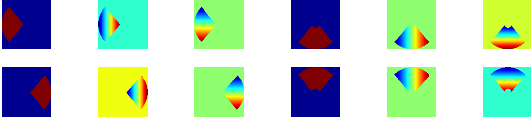
Figure 2. Piston, tip, and tilt basis used to recreate the PSF variations seen during the low wind effect on SPHERE. Each mode is normalized to 1 rad RMS (except the pistons). For the remainder of this paper, mode ‘1’ of this basis corresponds to the top left mode shown here (piston on the left segment). The remaining modes numerically follow from left to right, ending with mode ‘12’ shown in the bottom right of this figure (tip on the top segment).
