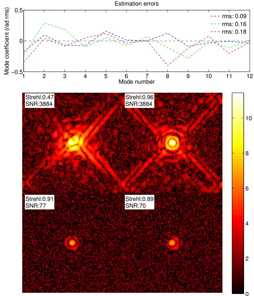
Figure 5. Top: residuals of LWE piston, tip, and tilt estimations from the actual modes, using Phase Diversity for 3 different scenarios (blue: long exposure object-estimation with focus diversity, green: object-estimation with higher diversity ( Z_{66} ), and red: assumed point source with focus-diversity). It can be seen the long exposure (blue) scenario performs the best, as indicated its RMS residual from the actual modes. Bottom: four panels of simulated VLT images, created from the phase projection of the estimated modes; they are described as follows: the upper two panels include no correction and long exposure Phase Diversity, respectively. The lower two panels include the higher diversity and assumed point source scenarios, respectively. From these images, the highest performance in terms of Strehl is clearly using the long exposure image. The bottom two images have diffraction rings that fall under the pedestal of the noise
