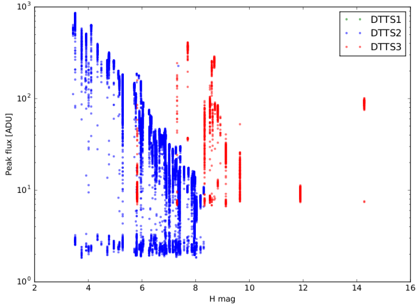
Figure 4. DTTS imager data, taken from SPHERE. The different colors correspond to different acquisition modes: blue points are taken in a mode optimized for bright stars while red points are suited for fainter stars; the green points represent an additional acquisition mode rarely used (and therefore explains the lack of points in this plot). The cloud of points around 2-3 ADU correspond to mis-detections, and we take this as the noise. Note: the values in this curve are subject to the inherent 20 nm PV focus on the DTTS imager, which results in a lower peak intensity than the true data shown here. After considering the noise floor and the data points adjusted for the 20 nm focus, we estimate a typical star has a SNR \sim 70 , and use this value for our analysis.
