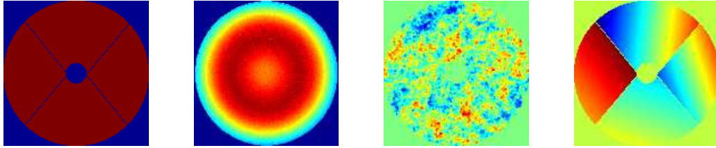
Figure 3. From left to right: VLT pupil, SPHERE apodization mask, assumed NCPA corresponding to 45 nm RMS WFE, and 1200 nm PV WFE low wind effect errors.
