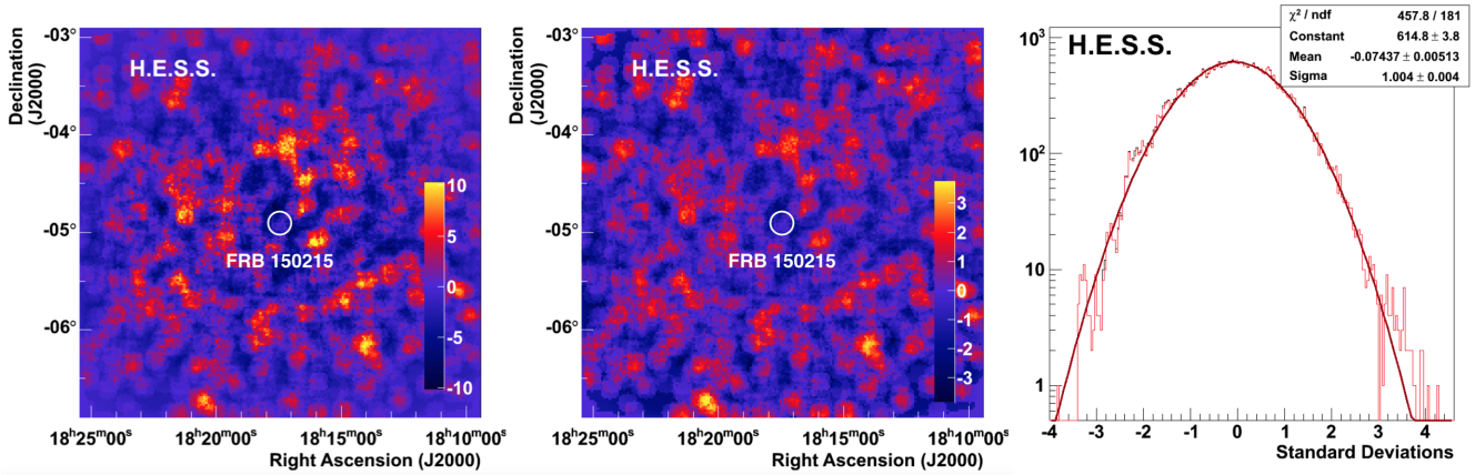
Figure 9. VHE \gamma -ray emission around the direction of FRB 150215 as observed with H.E.S.S (oversampling radius of 0.1^\circ ). The circle in the center has a diameter of 14.4' and denotes the width of the Parkes beam in which the burst has been observed. Left plot: \gamma -ray event counts exceeding the background expectation. Middle plot: Map of significances of the \gamma -ray emission using the formalism proposed by Li & Ma (1983). Right plot: Distribution of significances (black histogram) compared to the distribution obtained by excluding a circular region of 14.4' radius around the FRB position (red histogram). The red line and the shown parameters correspond to a Gaussian function fitted to the latter distribution.
