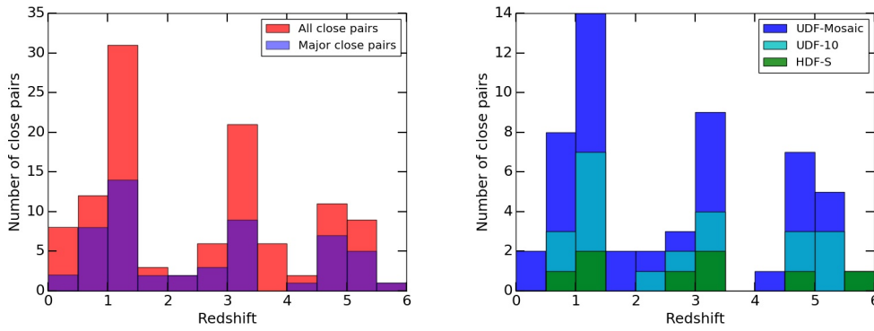
Fig. 2. Left: redshift distribution of all the galaxy close pairs (red) and the contribution of major close pairs (purple). Right: redshift histogram of the major close pairs showing the contribution of the different MUSE fields: UDF-Mosaic (dark blue), udf-10 (light blue), and HDF-S (green).
