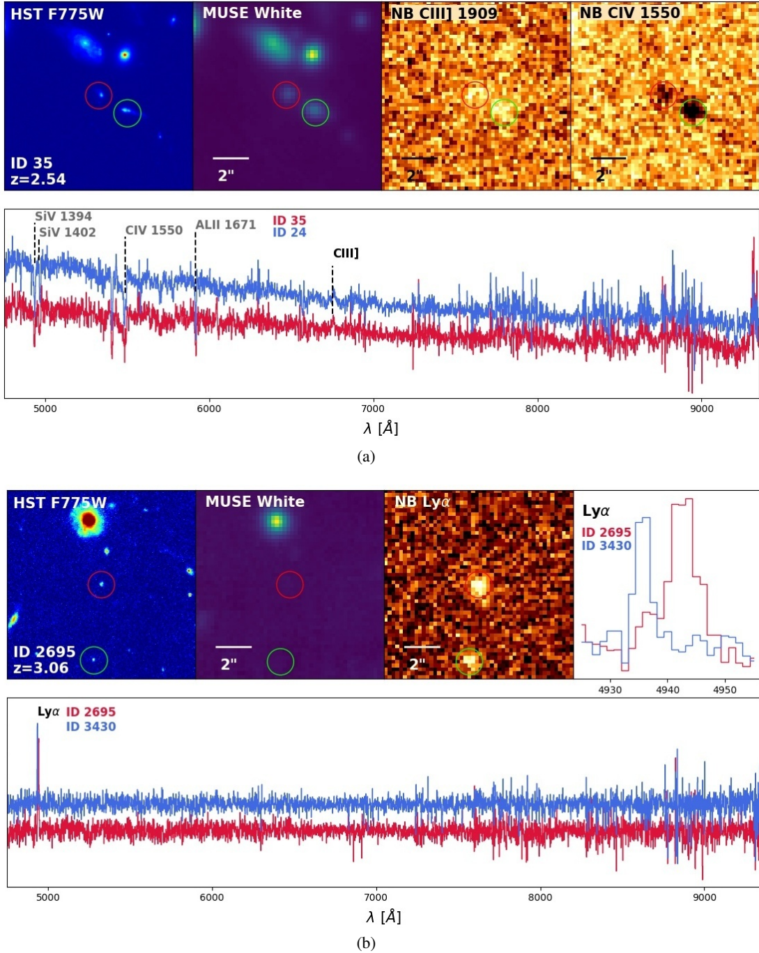
Fig. 4. Same as Fig. 3. Panel a: A close pair in udf-10 at a redshift of z = 2.54 with r_p \sim 15 kpc and \Delta v \sim 6 km s -1 . This is a good example of the galaxy pair population detected in the redshift desert bin. The two continuum-bright galaxies reveal a faint C III] \lambda\lambda 1907, 1909 emission line, as is shown in the first narrowband image, but are clearly identified thanks to their strong absorption lines. Panel b: A close pair of Ly \alpha emitters (LAE) in the UDF-Mosaic at z = 3.06 , one of the three close pairs with a rest-frame relative velocity higher than 300 km s -1 with \Delta v \sim 317 km s -1 and r_p \sim 31 kpc.
