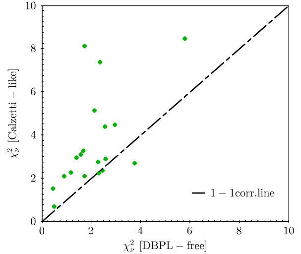
Figure 9. Comparison of \chi_v^2 values for z \sim 2 (U)LIRGs obtained with the DBPL-free recipe (x-axis) and the modified Calzetti recipe (y-axis). See text for further details.
