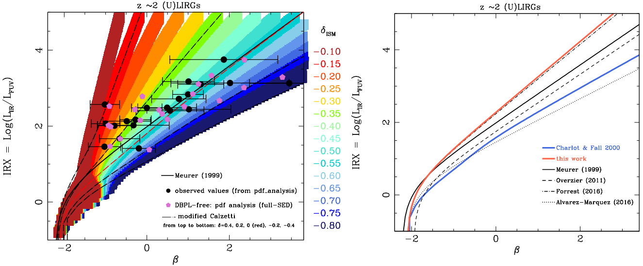
Figure 8. Left: observed estimates for the IRX- \beta of our z \sim 2 (U)LIRGs (filled black circles) compared to the predicted relations obtained through simulations color coded from blue to red as a function of increasing ISM slopes from -0.8 to -0.1. The thickness of the different colored stripes reflects the effect due to the assumed SFH, stellar population properties and different E(B-V)/A_V considered (see Tab. 1 for reference). These are also compared to the reference Meurer relation shown as solid black line and the modified Calzetti recipes, used in Salmon et al. (2016), with slopes ranging, from top to bottom, from +0.4 to -0.4. The red dot-long dashed line being that one corresponding to the assumption of a Calzetti et al. (2000) attenuation law ( \delta = 0 in the modified Calzetti recipe). The latter are used here as reference to show that in terms of UV-slope we cover the same range of values and they have been computed by assuming our reference SFH, namely, delay-tau model with input parameters as defined in Tab. 1. The magenta pentagons correspond to the estimates obtained through full SED-fitting under the assumption of DBPL-free model. Right: the IRX- \beta relation (red solid line) obtained by fitting the observed estimates from our z \sim 2 (U)LIRGs, is compared to that one obtained from simulations by assuming the CF00 model (blue solid line) and several reference relations from literature. Our relations appears to be in very good agreement with that one recently derived by Forrest et al. (2016).
