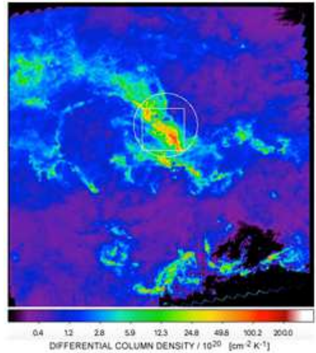
Figure 9. Differential column density, at a dust temperature of 13.2 K, over the 2.4^\circ \times 2.4^\circ field of the Hi-GAL tile at l \approx 224^\circ . The circle delineates a subregion used in the calculation of column density histograms shown in Fig. 8. The square represents the boundary of the cutout region shown in Fig. 10.
