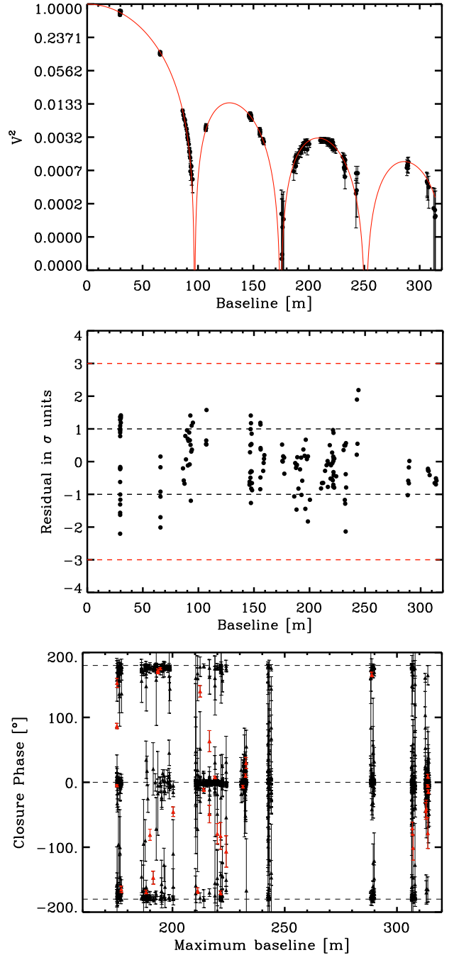
Fig. 1. Top and central panels: squared visibilities with the limb-darkening fit residuals ( top and central panels ) at the wavelength band 1.6004 \pm 0.0036 \mu\text{m} . The continuous line in the top panel corresponds to the limb-darkening fit whose parameters are reported in Table 3. The black horizontal dashed lines in the central panel correspond to the value of 1\sigma , and the red line shows the value of 3\sigma . Bottom panel: closure phase data points of \beta Oph (Table 2) for all the wavelengths. The red data correspond to closure phase departures larger than 3\sigma (see Fig. 2). The horizontal dashed lines in the bottom panel display the zero or \pm 180^\circ values.
