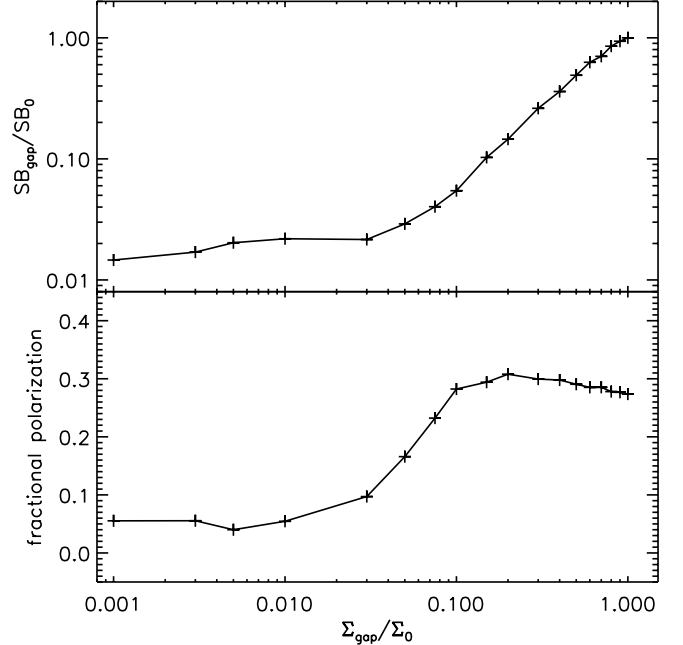
Figure 10. The contrast in scattered light total intensity (“Stokes I”, top panel) and fractional polarization (bottom panel) vs. the “depth” of the radial surface density depression, for a generic gap at the radial location of gap #2.
