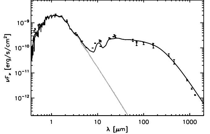
Figure 14. Spectral energy distribution of the radiative transfer model of the TW Hya disk compared with observations.
