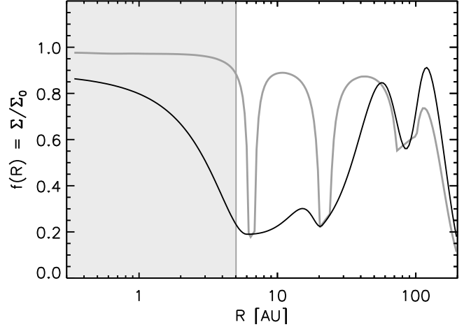
Figure 16. Comparison between our derived radial surface density depletion factor ( f(R) , black curve) and an implementation of the model of Duffell (2015) with three planets, approximately matching the depth of the gaps (grey curve). The innermost disk regions that are not well probed with our observations are masked. A distance of 54 pc has been assumed.
