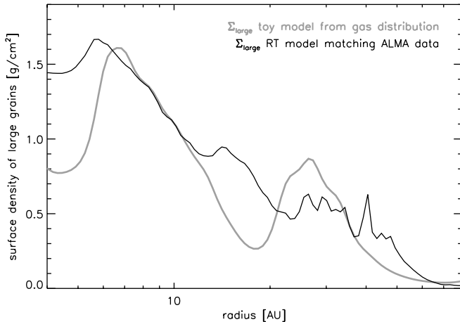
Figure 18. Toy model for the radial distribution of large dust derived from the gas distribution in our radiative transfer model (grey) compared to the radial distribution of large grains that reproduces the ALMA data (black). A distance of 54 pc has been assumed.
