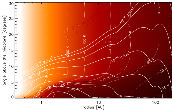
Figure 13. Density (full contours) and temperature (colors and dotted contours) of radiative transfer model. The black dashed line shows the \tau_{\text{scat}} = 2/3 surface in the H-band. A distance of 54 pc has been assumed.
