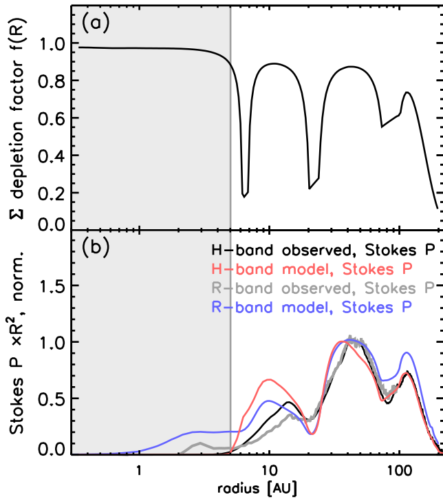
Figure 17. Equivalent to Fig. 11, but for the profile of the Duffell model in Fig. 16. A distance of 54 pc has been assumed.
