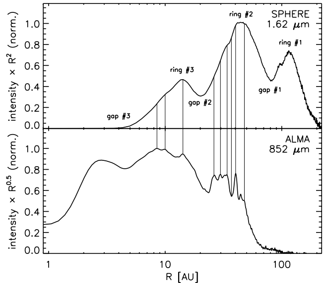
Figure 7. SPHERE H-band scattered light profile scaled with R^2 (top panel) and ALMA 852 \mu\text{m} continuum intensity profile scaled with \sqrt{R} . See Section 3.6 for a discussion. A distance of 54 pc has been assumed.
