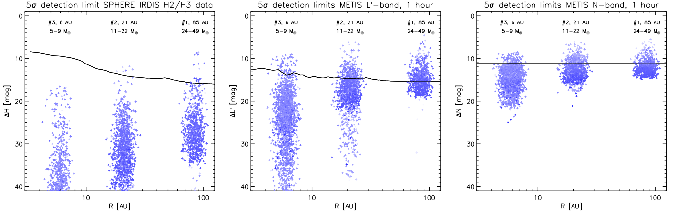
Figure 20. Synthetic photometry of the CD753 planet population from Mordasini et al. (2012) at 2 Myrs. The objects are color-coded according to physical size of the optically thick structure, with dark shades indicating compact and bright shades large objects. The black curves indicate the achieve detection limits of SPHERE (H-band, left panel) and the foreseen detection limits of METIS (L' and N-band, middle and right panel). A distance of 54 pc has been assumed.
