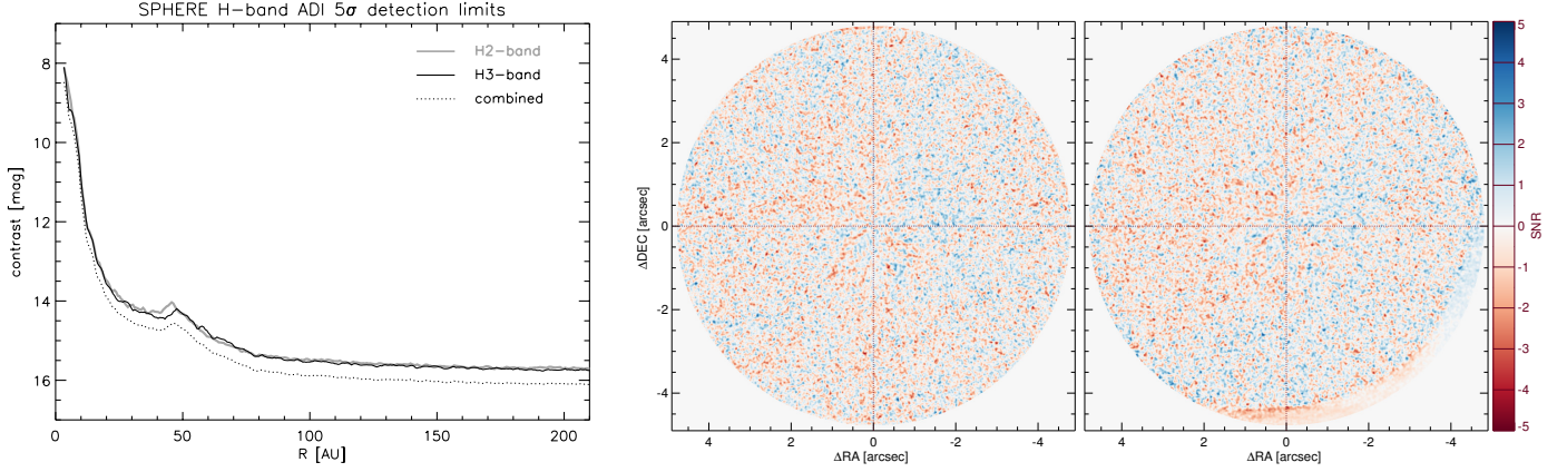
Figure 8. Summary of the IRDIS H2/H3-band angular differential imaging experiment. Left: achieved 5\sigma contrast curves. Right SNR maps obtained in the H2 and H3 filters. A distance of 54 pc has been assumed.
