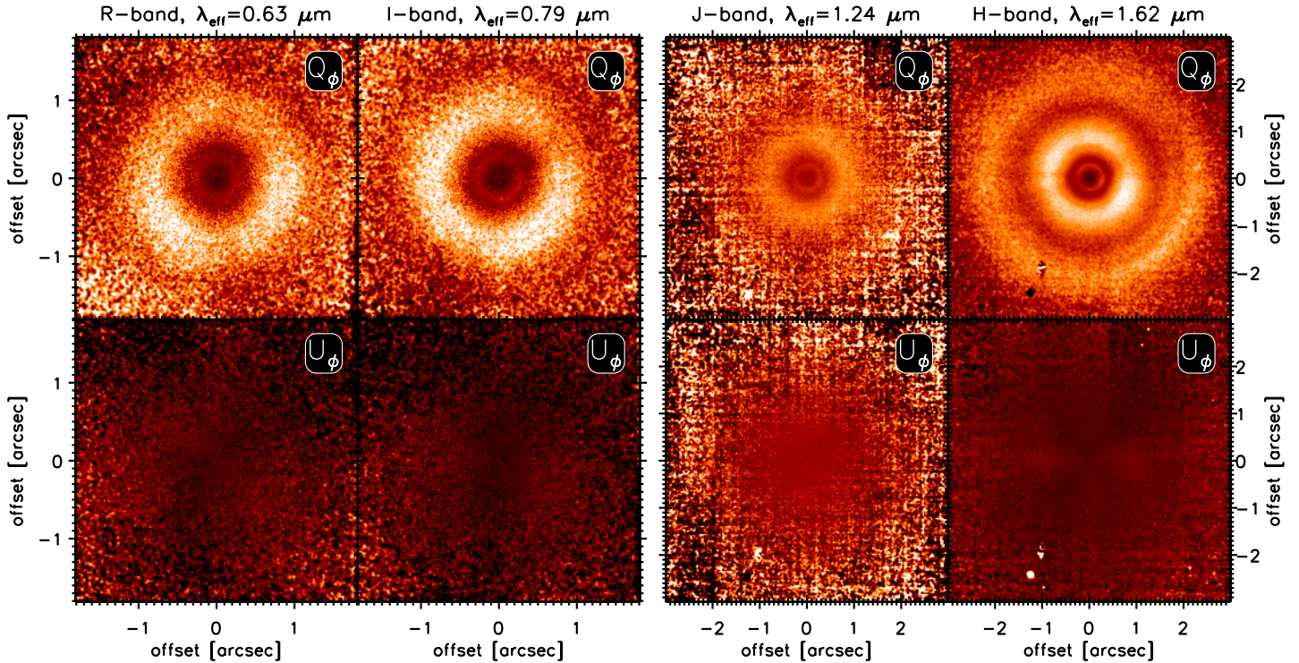
Figure 2. Q_\phi and U_\phi images of the TW Hya disk. North is up and East is to the left. The images have been scaled by R^2 to correct for the dilution factor of the stellar irradiation and each pair of Q_\phi and U_\phi images in a given band is displayed on the same linear stretch.
