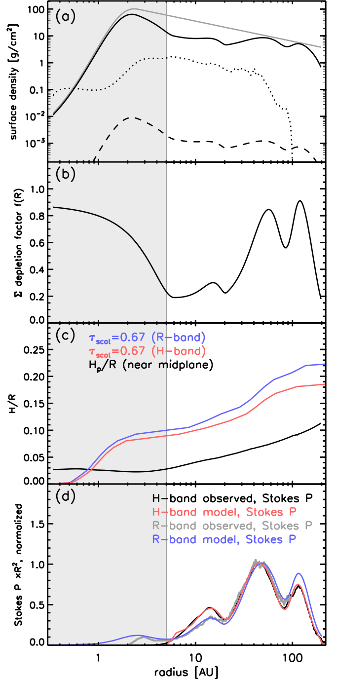
Figure 11. Overview of our radiative transfer model. Bottom panel: Black: H-band data, grey: R'-band data, red: convolved H-band model, blue: convolved R'-band model. The grey region at R \lesssim 5 au lies behind the coronagraph in the H-band observations. See Section 4.5 for details. A distance of 54 pc has been assumed.
