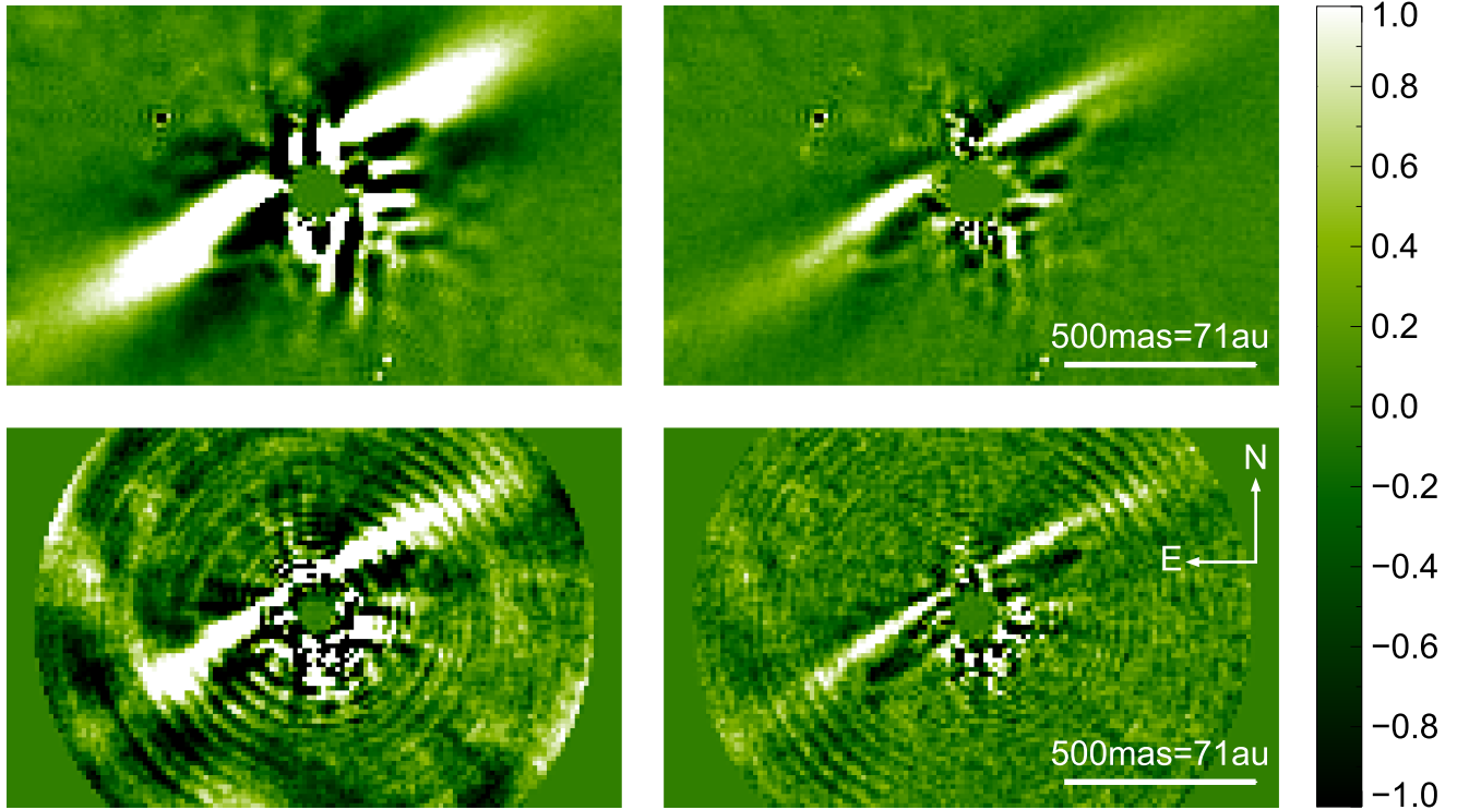
Figure 2. SPHERE detections of a scattered-light debris disk around the target HD 129590. Data from the IRDIS ( 1.6 \mu\text{m} ) and IFS ( 0.95\text{--}1.35 \mu\text{m} ) subsystems are shown on the top and bottom rows, respectively. In each case, the image is a co-add of the entire wavelength range of the subsystem. The left-hand images have six principal components subtracted, while on the right-hand side a more aggressive reduction is presented, where 20 principal components have been removed. In both cases, the reduction is full-frame treatment, where the entire field of view is considered simultaneously. The ringed structure observed in the IFS images is an artifact of the fast Fourier transform process used to rescale the various wavelength observations.
