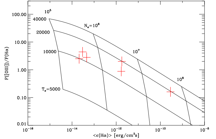
Fig. 13. Diagnostic diagram based on H\alpha line emissivities \epsilon(H\alpha) and [O III]/ H\alpha line ratios assuming an abundance ratio N_{O^{+2}}/N_{H^+} = 5 \times 10^{-4} . The crosses give the values for the H\alpha clouds with [O III]/ H\alpha -ratios from HST.
