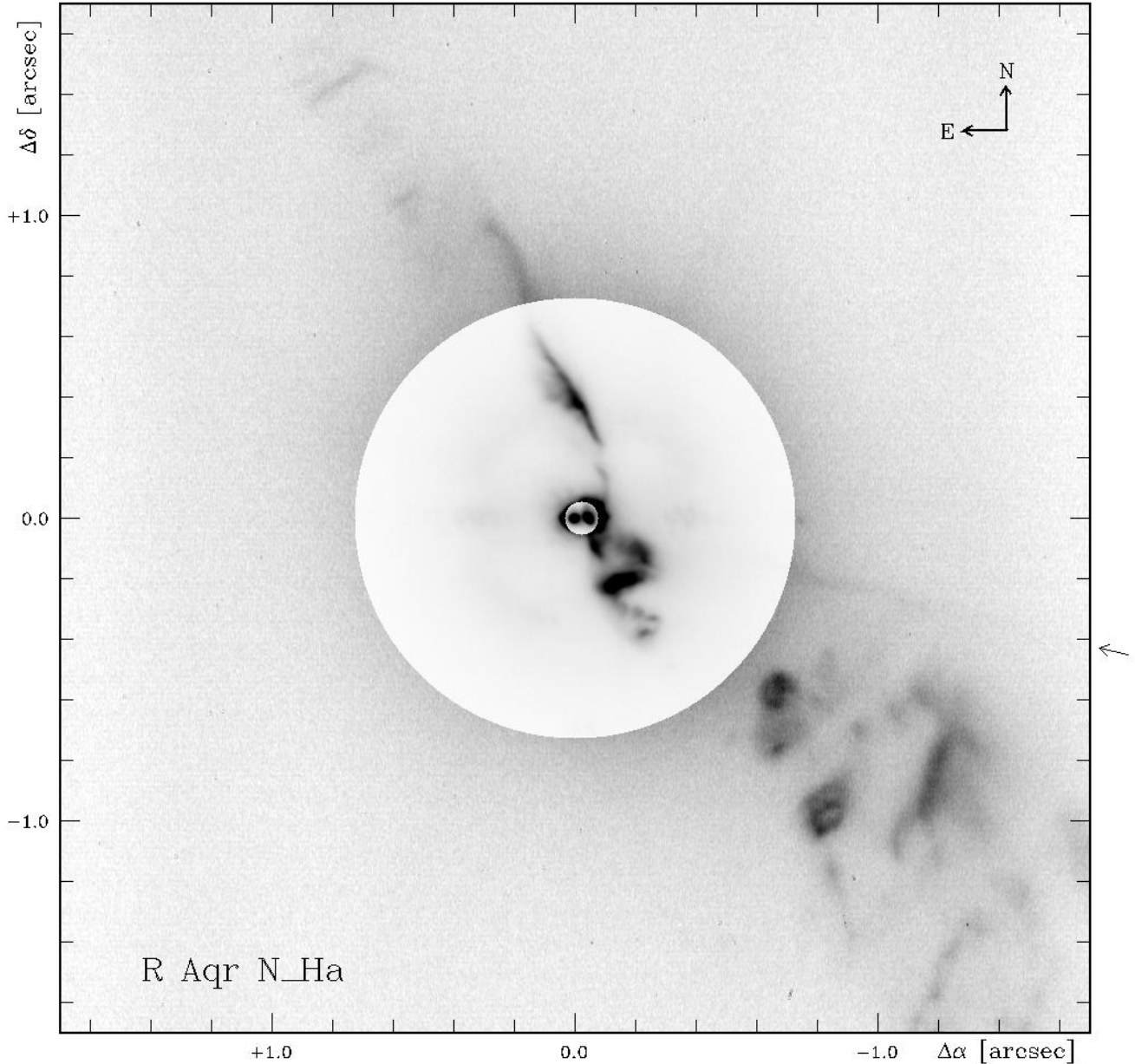
Fig. 6. Map of the SPHERE/ZIMPOL H\alpha line observation of R Aqr taken in the N\_Ha ( FWO ) filter on Oct. 11, 2014. The field is divided into three different gray scale regions ranging from 0 to 1000 \text{ct pix}^{-1} \text{ frame}^{-1} for the central binary, 0 to 100 for the inner jet region r_{\text{RG}} < 0.72'' , and 0 to 10 for the outer jet region r_{\text{RG}} > 0.72'' . The red giant is at the zero point of the coordinate system. There is a small angle offset of 2 deg of the sky N orientation in a counter-clockwise direction with respect the (vertical) y -direction. A weak instrumental spike from a telescope spider is present at a position angle of about -105^\circ indicated by a small arrow outside the frame.
