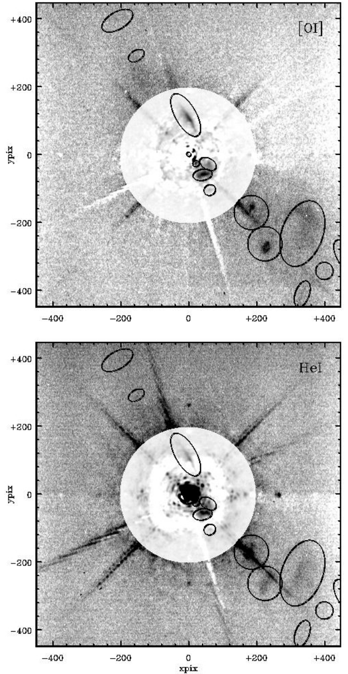
Fig. 11. SPHERE/ZIMPOL OI_630- and He-I-filter observations of the R Aqr jet. The emission of the red giant is strongly reduced by subtracting a scaled CntHa filter image. The gray scale tables are multiplied by a factor of ten for the inner r_{RG} < 0.72'' region.
