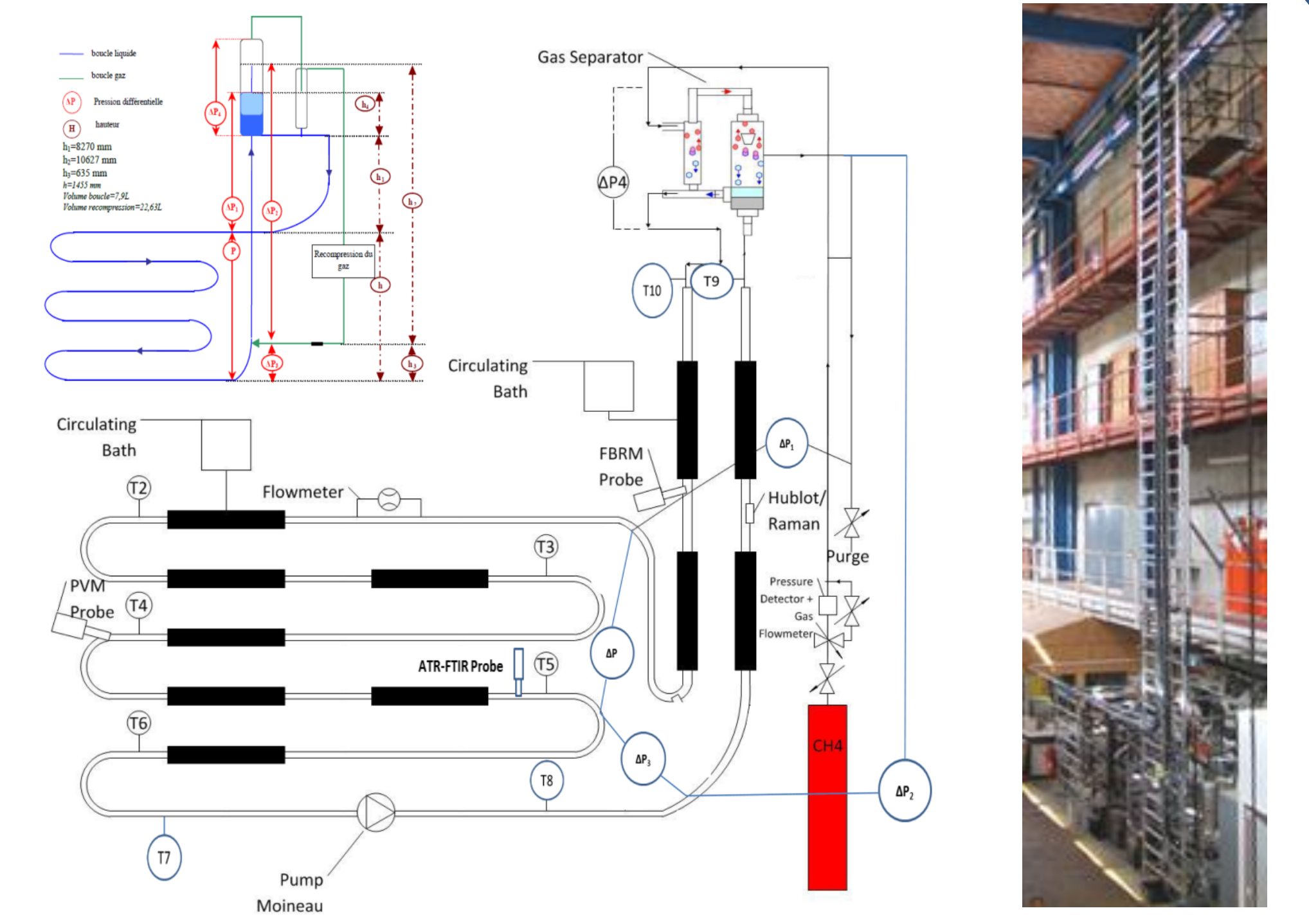
Figure 3 – Archimède flowloop photos and schemas [1-2-3].
