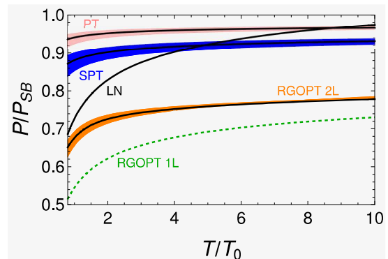
FIG. 6. P/P_{SB}(T/T_0) in high- T approximation for N = 4 , g(M_0 = 2\pi T_0) = 1 , and scale variation 1/2 < \alpha < 2 . Pink range: PT; blue range: SPT; black: LN; orange range: two-loop RGOPT; green dashed line: one-loop RGOPT.
