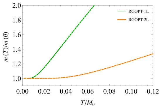
FIG. 4. The normalized thermal optimized masses, \bar{m}(T)/\bar{m}(0) , as a function of the temperature T (normalized by M_0 ) for N = 4 , g(M_0) = 1 = g_{LN}(M_0)/2 , and at the central scale choice \alpha = 1 , in the RGOPT at one- and two-loop cases. (NB for this coupling choice the LN thermal mass is identical to the RGOPT one-loop one).
