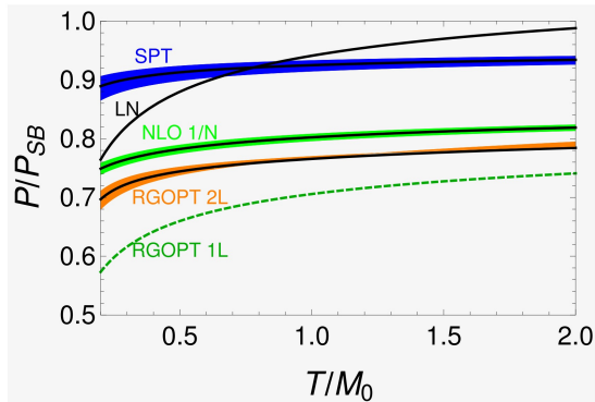
FIG. 7. P/P_{SB}(T/M_0) in high- T approximation for N = 4 , g(M_0) = 1 = g_{LN}(M_0)/2 and scale variation 1/2 < \alpha < 2 . Same captions as in Fig. 6, with added comparison to 1/N NLO pressure (green range).
