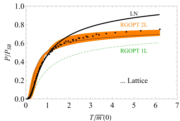
FIG. 9. P/P_{SB} as a function of the temperature T (normalized by the T = 0 mass gap \bar{m}(0) ) for N = 3 : LN, one- and two-loop RGOPT for g(M_0) = g_{LN}(M_0) = 2\pi and scale variation 1/2 \leq \alpha \leq 2 , when using RG optimized running given by Eq. (6.5), compared with lattice simulations (taken from Ref. [31]). NB lattice data have been conveniently rescaled on vertical axis from P/T^2 in Ref [31] to P/P_{SB} (i.e., for N = 3 this corresponds to a scaling factor of \pi/3 ).
