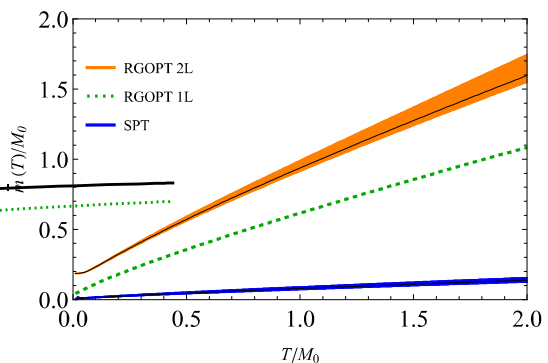
FIG. 3. Thermal masses as a function of the temperature (both quantities normalized by the reference scale M_0 ) for scale variations 0.5 \leq \alpha \leq 2 , N = 4 and g(M_0) = g_{LN}(M_0)/2 = 1 . We compare the results for the RGOPT (one- and two-loop cases) and the SPT. (NB for this coupling choice the LN thermal mass is identical to the RGOPT one-loop one). Within the two-loop RGOPT and SPT, the shaded bands have the lower edge for \alpha = 0.5 and the upper edge for \alpha = 2 . The thin line inside the shaded bands is for \alpha = 1 .
