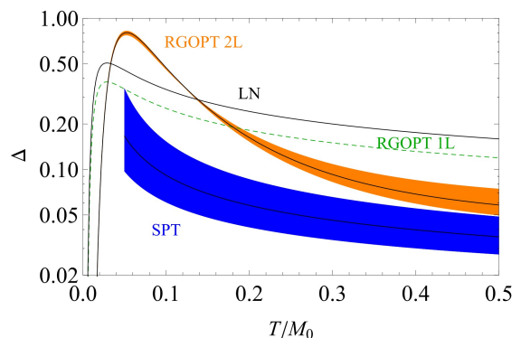
FIG. 10. The interaction measure \Delta as a function of the temperature T (normalized by M_0 ) for N = 4 and g(M_0) = 1 = g_{LN}(M_0)/2 , with scale variation 0.5 \leq \alpha \leq 2 , using the standard two-loop running coupling given by Eq. 5.16). Within the two-loop RGOPT and SPT, the shaded bands have the lower edge for \alpha = 0.5 and the upper edge for \alpha = 2 . The thin line inside the shaded bands is for \alpha = 1 . (Logarithmic scale is used).
