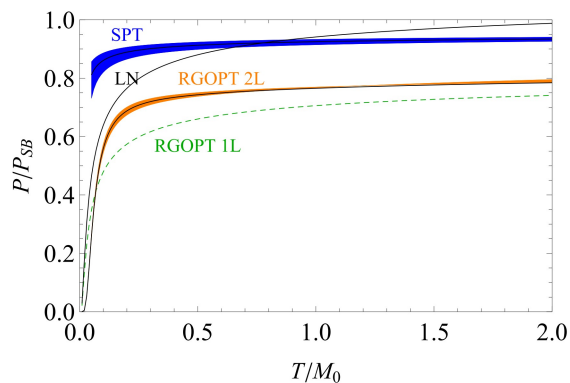
FIG. 5. P/P_{SB} as function of the temperature T (normalized by M_0 ) for N = 4 and g(M_0) = 1 = g_{LN}(M_0)/2 , with scale variation 0.5 \leq \alpha \leq 2 . Within the two-loop RGOPT and SPT, the shaded bands have the lower edge for \alpha = 0.5 and the upper edge for \alpha = 2 . The thin line inside the shaded bands is for \alpha = 1 . (NB the line thickness of one-loop RGOPT and LN is only for visibility at the figure scale and does not correspond to any actual scale dependence since those approximations are exactly scale invariant.)
