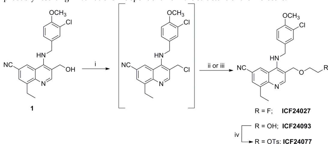
Scheme 1. Synthetic pathway to the novel 2-fluoroethoxy derivative ICF24027 and the tosylate precursor ICF24077 . (i) SOCl_2 , 30 min, rt; (ii) 2-fluoroethanol, DMF, 80 °C, 30 h for ICF24027 ; (iii) ethylene glycol, DMF, 80 °C, 16 h for ICF24093 ; (iv) p -toluenesulfonyl chloride, NEt_3 , DMAP, CH_2Cl_2 , rt, 20 h.
