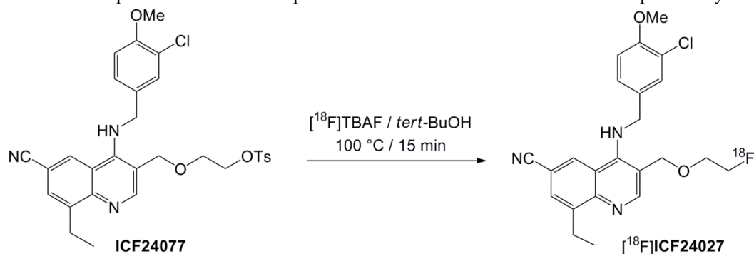
Scheme 2. ^{18}F -Radiolabelling of [^{18}F]\text{ICF24027}
