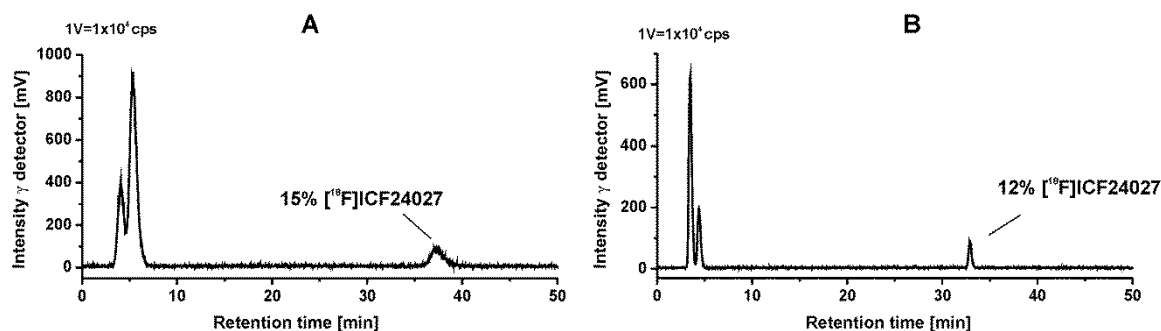
Figure 5. Representative radio chromatograms of a mouse brain sample of [ ^{18}\text{F} ]ICF24027 30 min p.i. A: Micellar chromatography (conditions: Reprisil-Pur C18-AQ, 250x4.6 mm, gradient: 3-30-3% 1-PrOH/100 mM SDS aq, 10 mM \text{Na}_2\text{HPO}_4 aq; flow: 0.75 mL/min). B: Reversed phase chromatography (conditions: Reprisil-Pur C18-AQ, 250x4.6 mm, gradient: 10-90-10% ACN/20 mM \text{NH}_4\text{OAc} aq; flow 1.0 mL/min).
