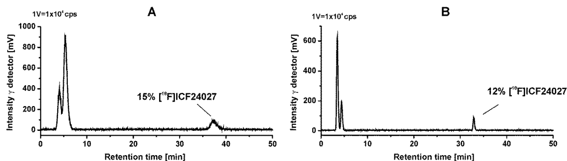
Figure 5. Representative radio chromatograms of a mouse brain sample of ^{18}\text{F} ICF24027 30 min p.i. A: Micellar chromatography (conditions: Reprosil-Pur C18-AQ, 250x4.6 mm, gradient: 3-30-3% 1-PrOH/100 mM SDS aq., 10 mM \text{Na}_2\text{HPO}_4 aq.; flow: 0.75 mL/min). B: Reversed phase chromatography (conditions: Reprosil-Pur C18-AQ, 250x4.6 mm, gradient: 10-90-10% ACN/20 mM \text{NH}_4\text{OAc} aq.; flow 1.0 mL/min).
