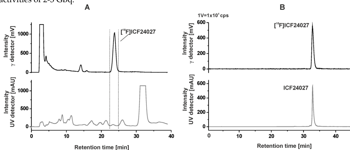
Figure 2. A: Semi-preparative radio- and UV-HPLC chromatograms of [ ^{18}\text{F} ]ICF24027 (conditions: Reprosil-Pur C18-AQ, 250x10 mm, 62% ACN/20 mM \text{NH}_4\text{OAc}_{\text{aq}} , 3.0 mL/min). B: Analytical radio- and UV-HPLC chromatograms of the final product of [ ^{18}\text{F} ]ICF24027 spiked with the nonradioactive reference ICF24027 (conditions: Reprosil-Pur C18-AQ, 250x4.6 mm, gradient with eluent mixture of ACN/20 mM \text{NH}_4\text{OAc} aq., 1.0 mL/min).
