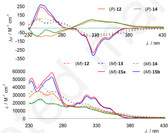
Figure 5. UV-vis and ECD spectra of enantiomers ( P ) and ( M )- 12 , ( M )- 13 , ( P ) and ( M )- 14 and the two enantiopure diastereomers ( M )- 15a and ( M )- 15b ( C \sim 5.10^{-5} \text{ M} in \text{CH}_2\text{Cl}_2 ).
