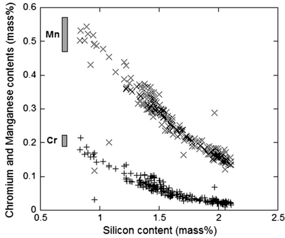
Fig. 11—Correlation between individual measurements in silicon vs chromium and manganese contents. The rectangles represent the intrinsic variability of each measurement, the length of the horizontal side is 2\sigma for silicon (about 0.05 mass pct) and that of the vertical side 2\sigma for either chromium (about 0.03 mass pct) or manganese (about 0.1 mass pct).
