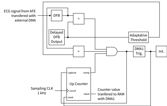
Figure 3: Hardware detection of RR intervals
