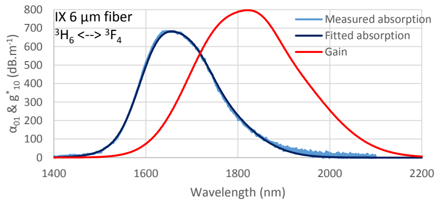
Figure 2: Core absorption and gain coefficients for the IX6 fiber used in the simulations.
