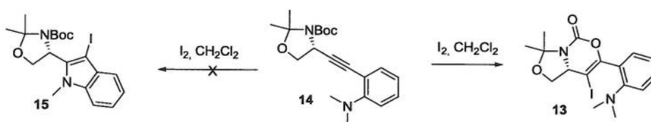
Fig. 10 Nucleophilic attack of Boc group under Larock's iodocyclization condition
