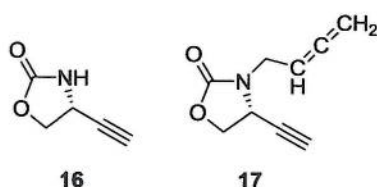
Fig. 12 4-Ethynyloxazolidin-2-one derivatives 16 and 17 as ethynylglycine synthons
