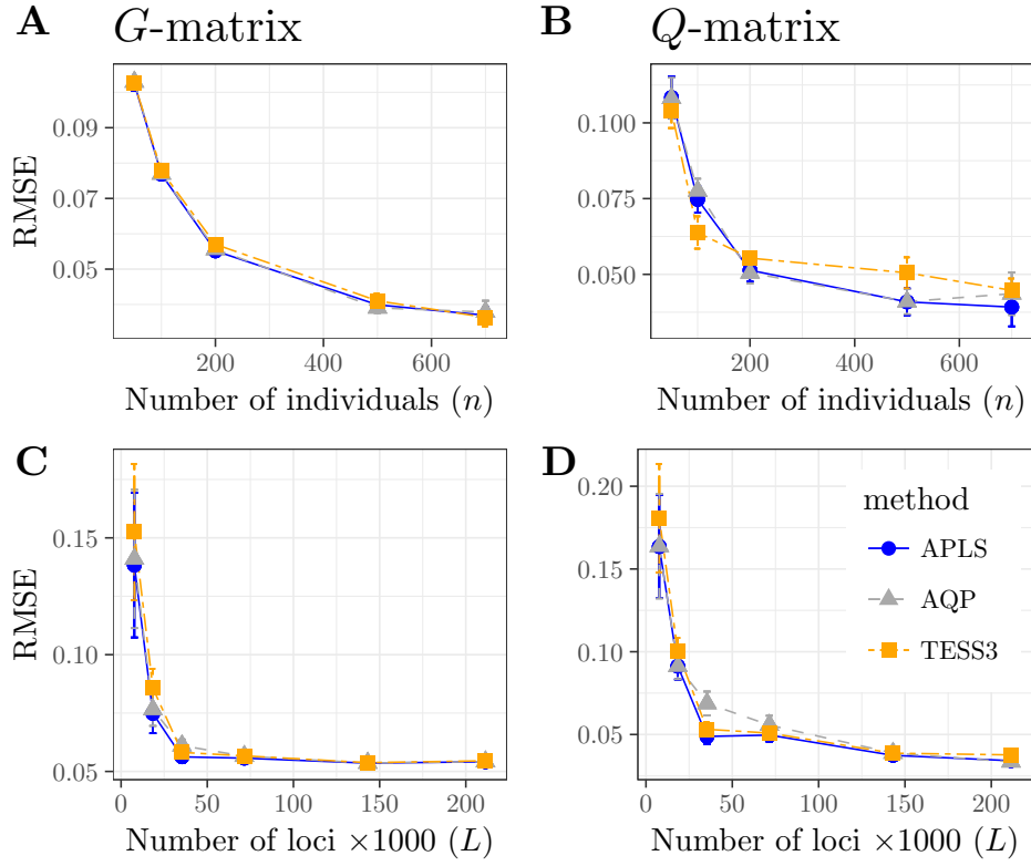
FIG 1. Root Mean Squared Errors (RMSEs) for the G and Q matrix estimates. Simulations of spatially admixed populations. A-B) Statistical errors for APLS, AQP and tess3 estimates as a function of the sample size, n ( L \sim 10^4 ). C-D) Statistical errors for APLS, AQP and tess3 estimates as a function of the number of loci, L ( n = 200 ).
