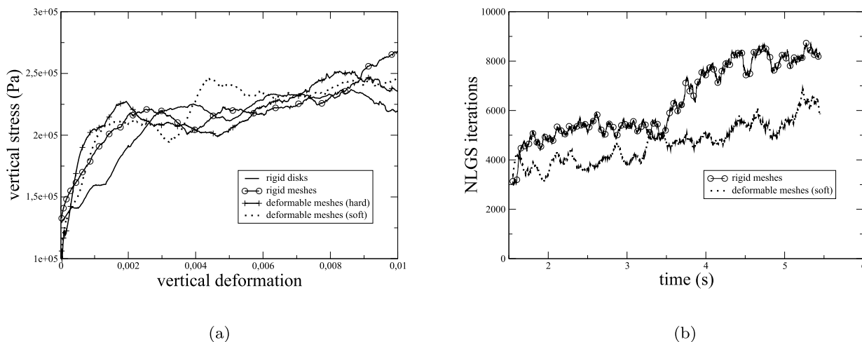
Fig. 7. Bi-axial test: (a) stress–strain curve, (b) NLGS iterations evolution during the compression phase.
