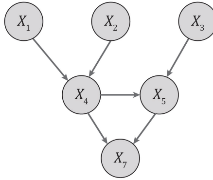
Figure 6: An example of Bayesian Probabilistic Network (Gonzva, M.)
