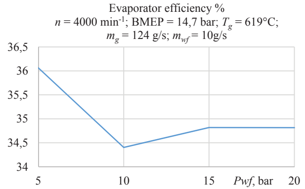
Fig. 17. Evaporator efficiency.
