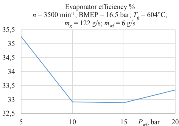
Fig. 16. Evaporator efficiency.
