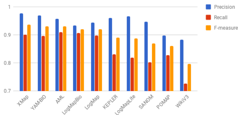
Fig. 5. KEPLER evaluation metrics among other pioneering systems for LargeBio track.
