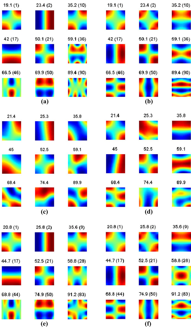
Fig. 3 Mode shapes and resonant frequencies (in kHz) measured ( c , d ), computed ones paired using the initial guess elastic constants estimated using Guitard and El Amri (1987) ( a , b ), and final computed ones after identification ( e , f ) on R and L faces, respectively. Values in parentheses correspond to the theoretically computed mode number
