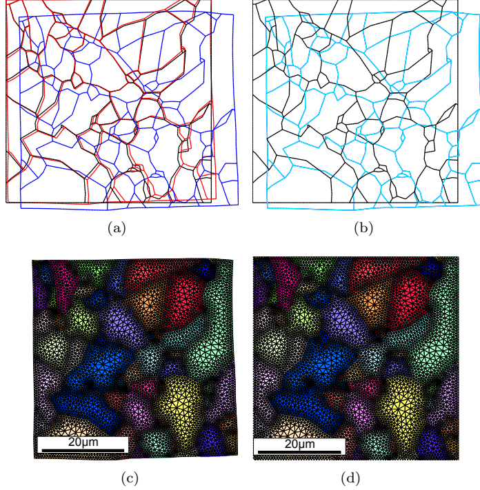
Figure 6: Backtracked reference configuration. (a) Grain boundaries of \Omega_{ref}^{(3)} is shown in red lines. (b) Grain boundaries of \Omega_{def}^{exp} is shown in cyan lines. For comparison purposes, \Omega_{ref}^{exp} is shown in black lines and \Omega_{def}^{exp} is shown in blue lines in both figures. Note that \Omega_{def}^{(3)} coincides with \Omega_{def}^{exp} in (b). (c) \Omega_{ref}^{(3)} is shown as an orientation map. (d) \Omega_{ref}^{exp} is shown as an orientation map for comparison purposes
