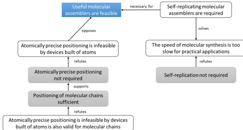
Fig. 4: Molecular assembler feasibility argument map
