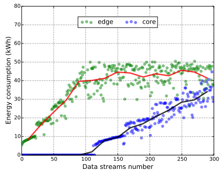
(a) Energy consumption with resolution 360p.
