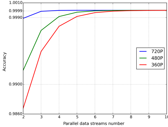
Figure 8: Application’s accuracy (from the statistical formula detailed in [17]).
