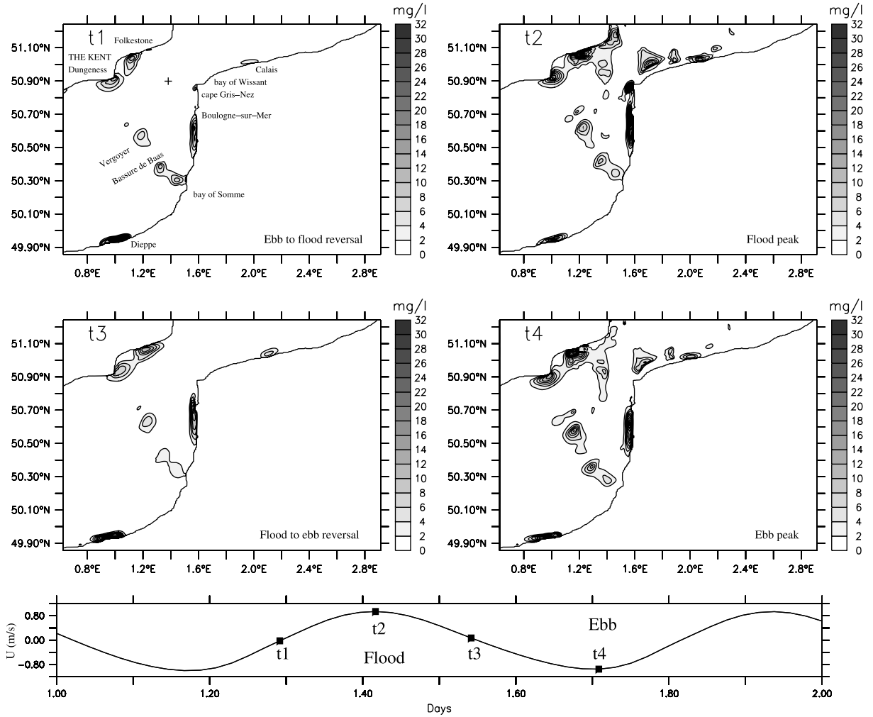
Figure 4. Predicted fields of total SSC 40 cm below the free surface at times of current peaks (t2, t4) and slack waters (t1,t3) of a mean tidal cycle in the centre of the inner domain ( \lambda = 1^{\circ}400\text{ E} , \phi = 50^{\circ}900\text{ N} ), localized by + in the top left slide.
