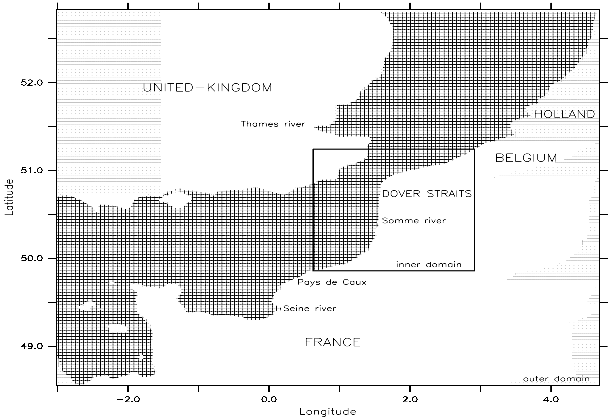
Figure 2. Outer and inner computational domains.
