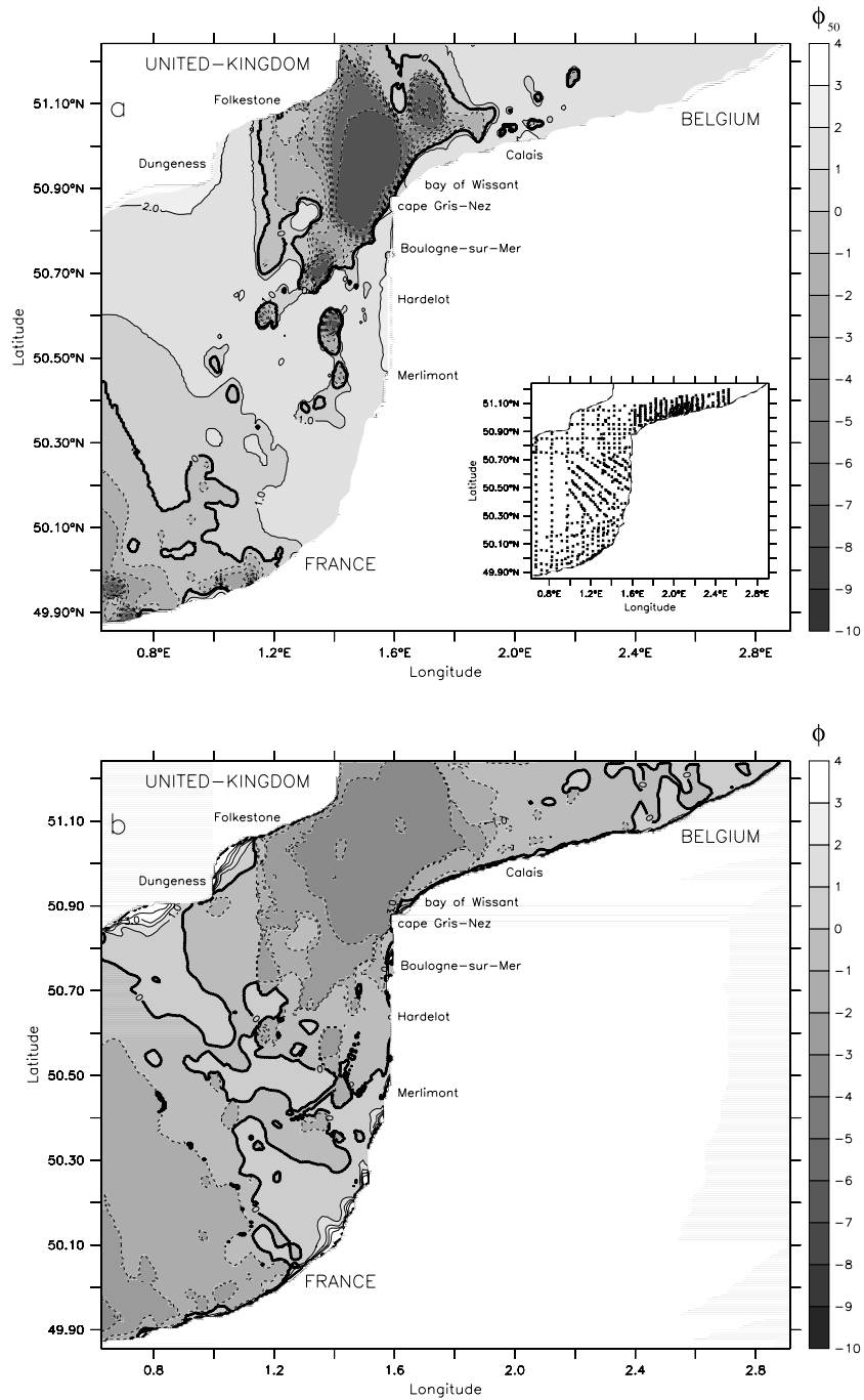
Figure 3. (a) Median sieve diameter expressed in the Wentworth's grain-size scale \Phi_{50} = -\log_2(d_{50}) (with d_{50} in mm) in the inner domain. The right-bottom sheet represents the geographic distribution of the 679 "RCP 378 Benthos de la Manche" grab samples in the Dover Strait. (b) Critical incipient motion diameter in the Wentworth's scale inferred from the highest tidal conditions in the inner domain.
