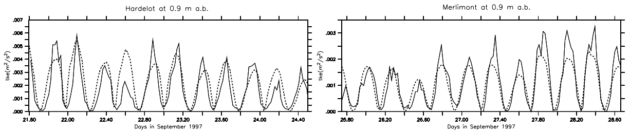
Figure 8. Measured (black-line) and computed (dotted-line) time series of the turbulent kinetic energy at 0.9 m above the bottom at the Haredlot and Merlimont sites.
