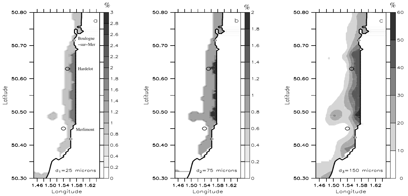
Figure 5. Proportions of each of the first three grain-size classes in the surroundings of the Harelot site.
