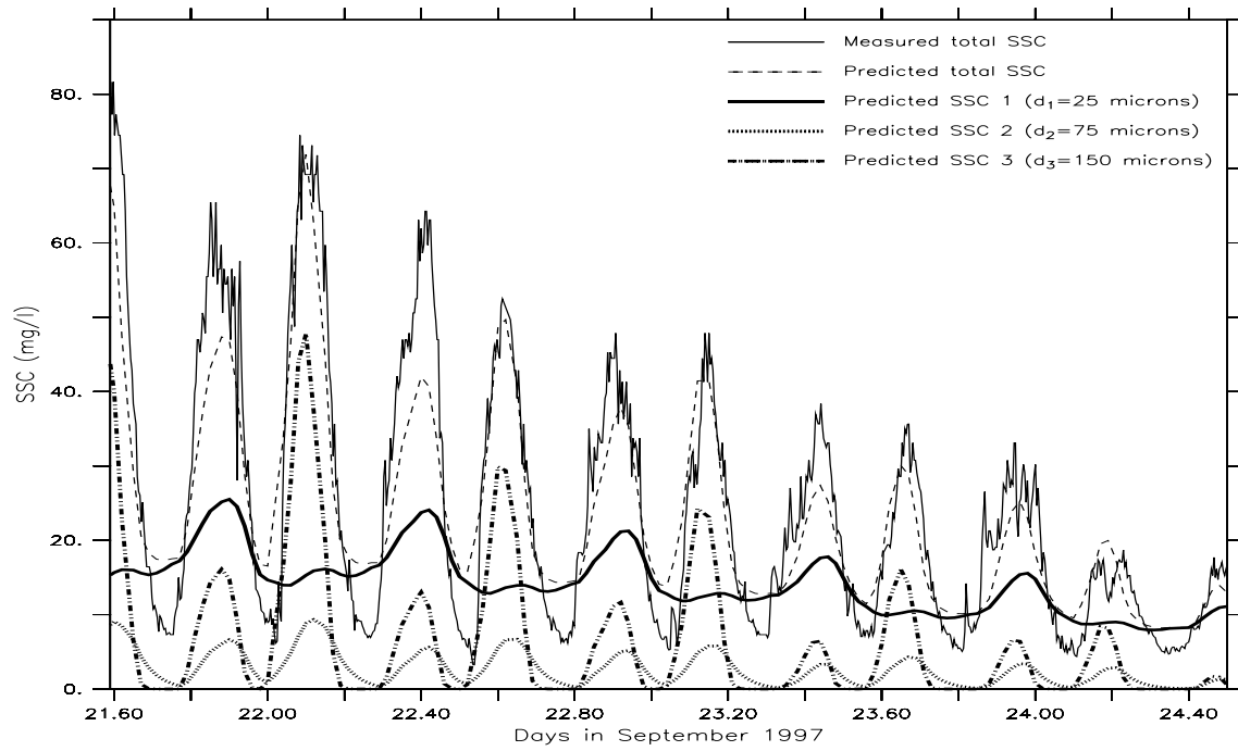
Figure 9. Measured and computed time series of the total SSC and the SSC of the first three classes with diameters d_1 = 25 \mu\text{m} , d_2 = 75 \mu\text{m} and d_3 = 150 \mu\text{m} involved in suspension at 5 m above the bottom at the Hardelot site.
