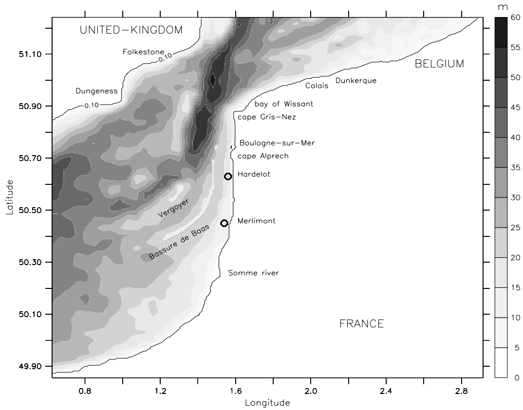
Figure 1. Bathymetry of the Dover Strait taking into account the mean sea level.
