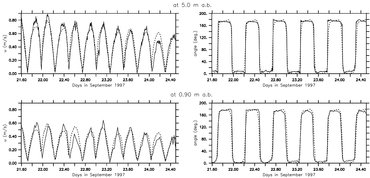
Figure 6. Measured (black-line) and computed (dotted-line) time series of the speed and direction (clockwise from the North) at 0.9 and 5 m above the bottom at the Harelot site.
